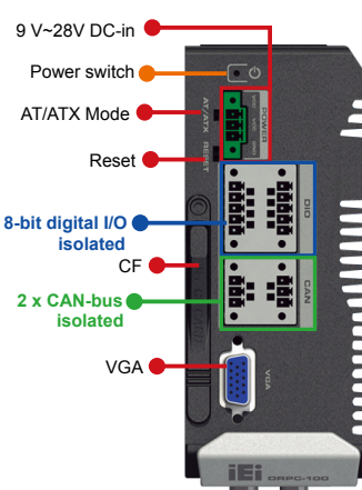
DRPC-100 Top Side View
