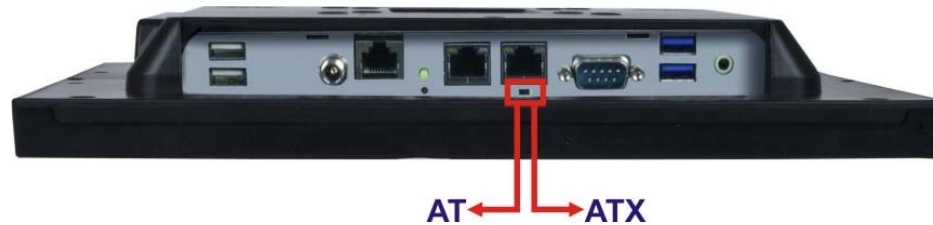
Figure 3-14: AT/ATX Switch Location
