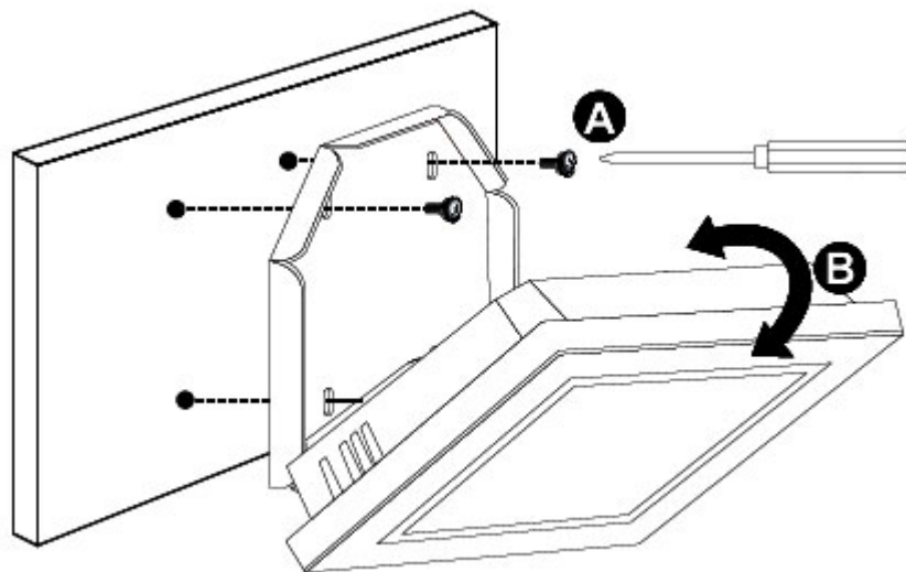
Figure 3-34: Secure V-Stand to Mounting Area
