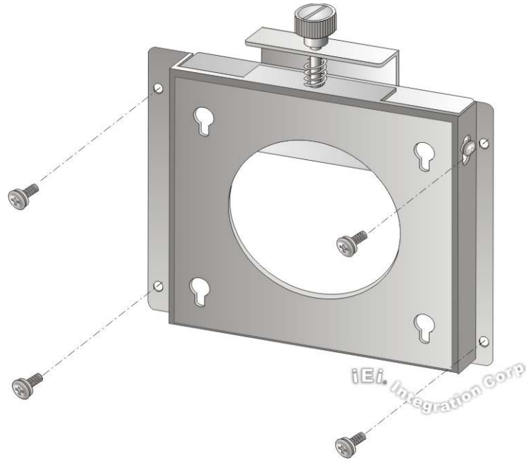
Figure 3-16: Wall-mounting Bracket
