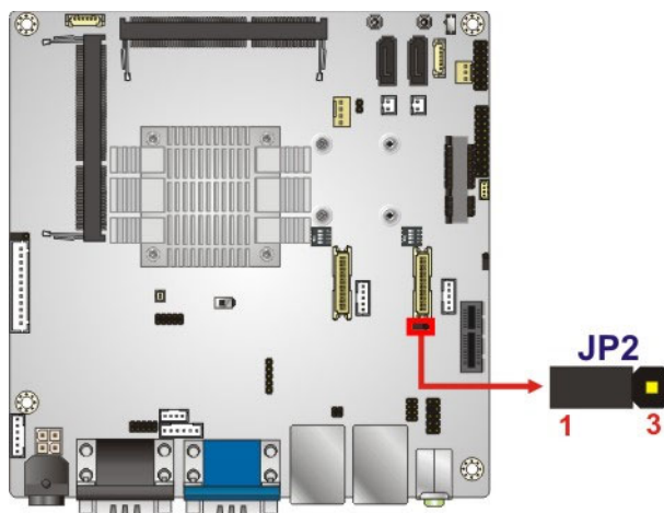
Figure 4-16: LVDS2 Voltage Selection Jumper Location
