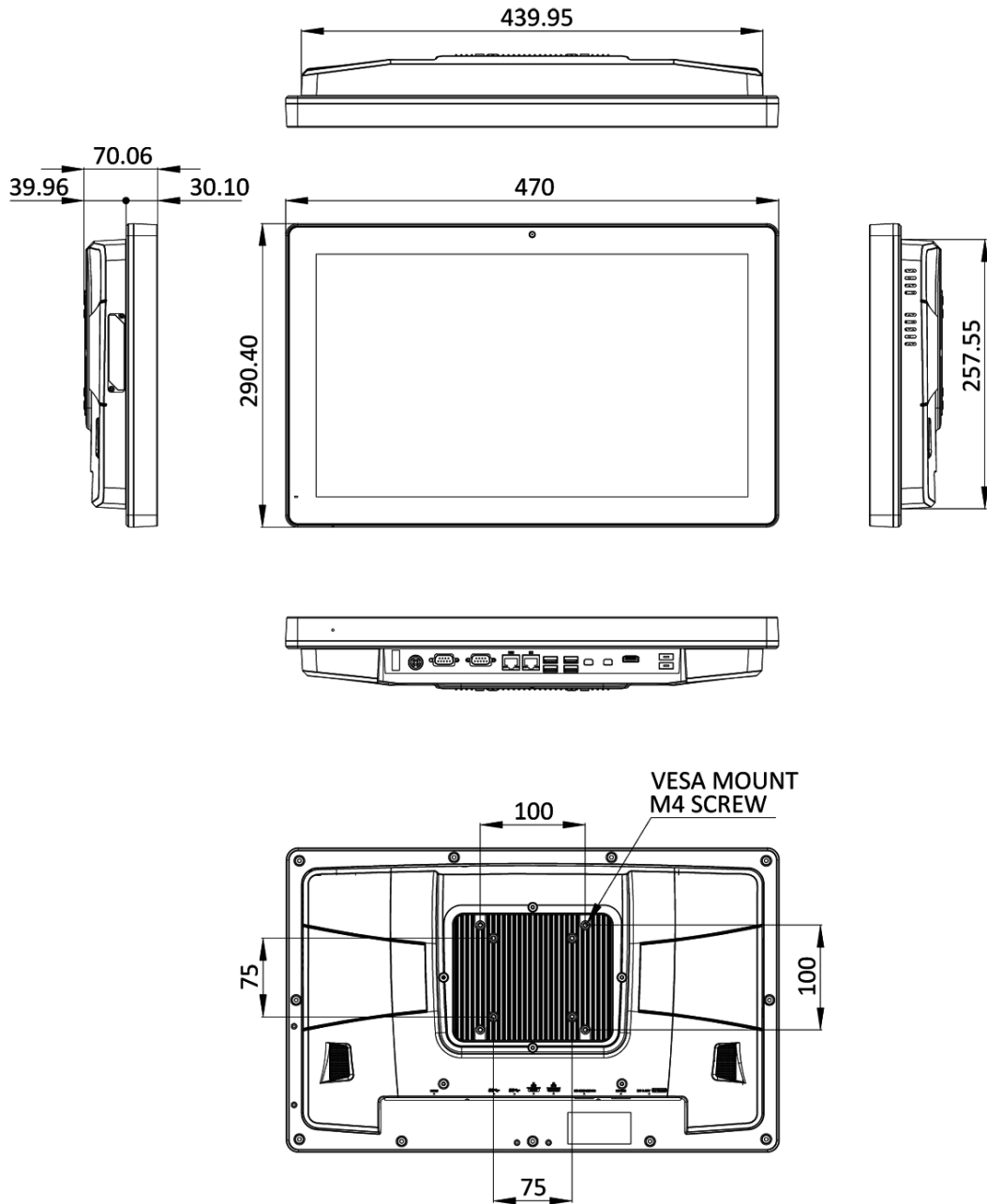
Figure 1-7: AFL3-W19C-ULT3 Dimensions (mm)
