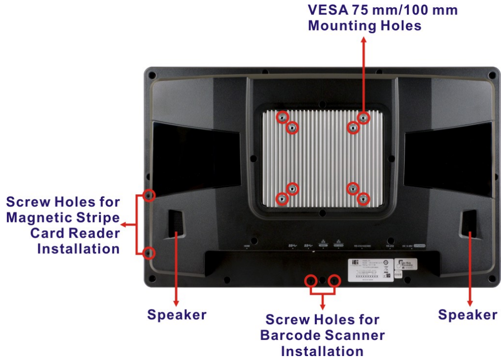
Figure 1-5: AFL3-W19C-ULT3 Rear View
