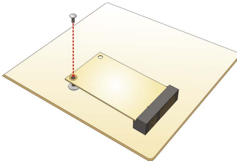
Figure 3-13: Securing the mSATA Module
