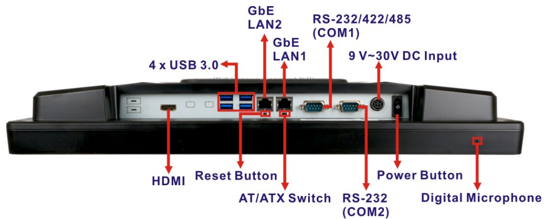
Figure 1-4: AFL3-W19C-ULT3 Bottom Panel
