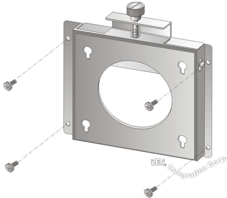
Figure 3-21: Wall-mounting Bracket
