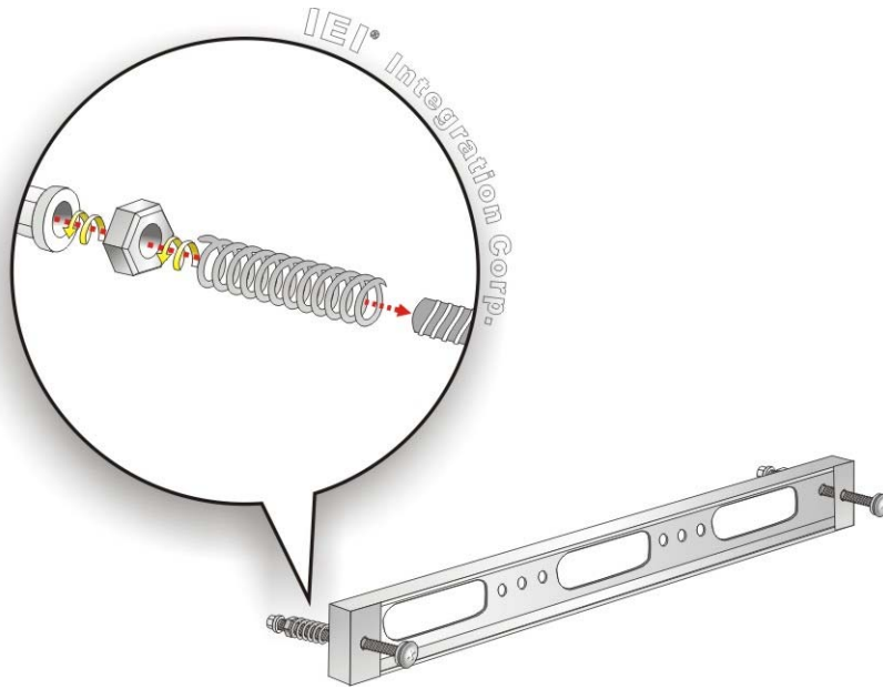
Figure 3-26: Panel Mounting Kit Installation
