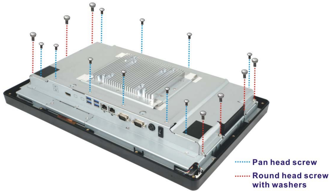
Figure 3-4: AFL3-W19C-ULT3 Aluminum Cover Retention Screws
