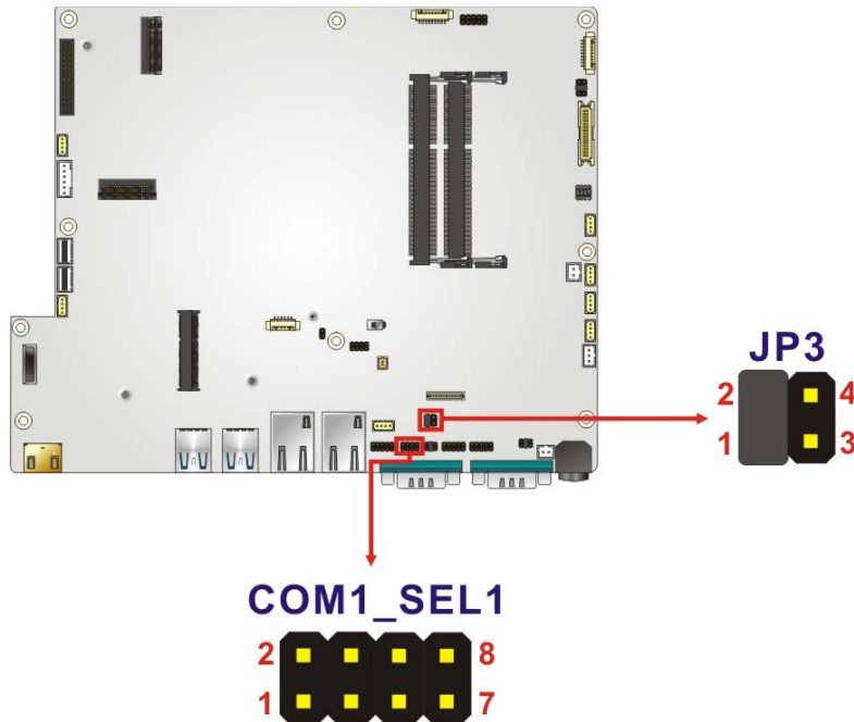
Figure 3-18: RS-232/422/485 Selection Jumper Locations
