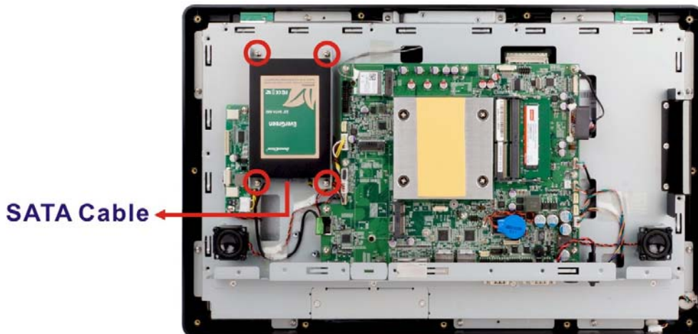
Figure 3-16: HDD Installation
