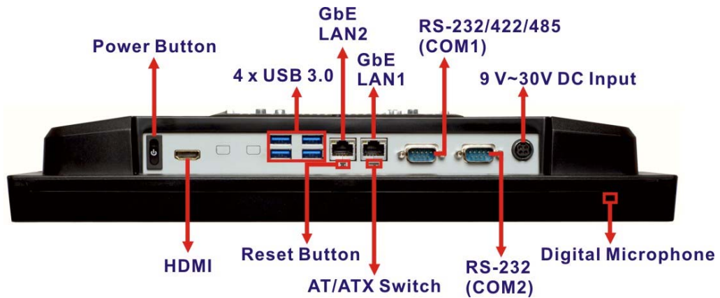
Figure 1-3: AFL3-W15C-ULT3 Bottom Panel
