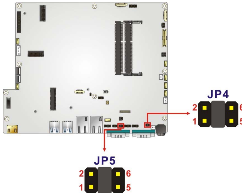
Figure 3-17: DB-9 Serial Port Pin 9 Setting Jumper Locations
