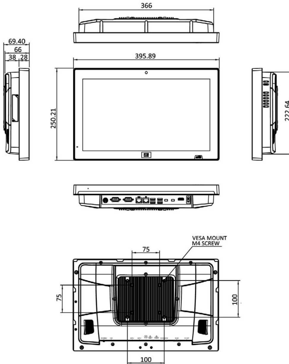
Figure 1-6: AFL3-W15C-ULT3 Dimensions (mm)
