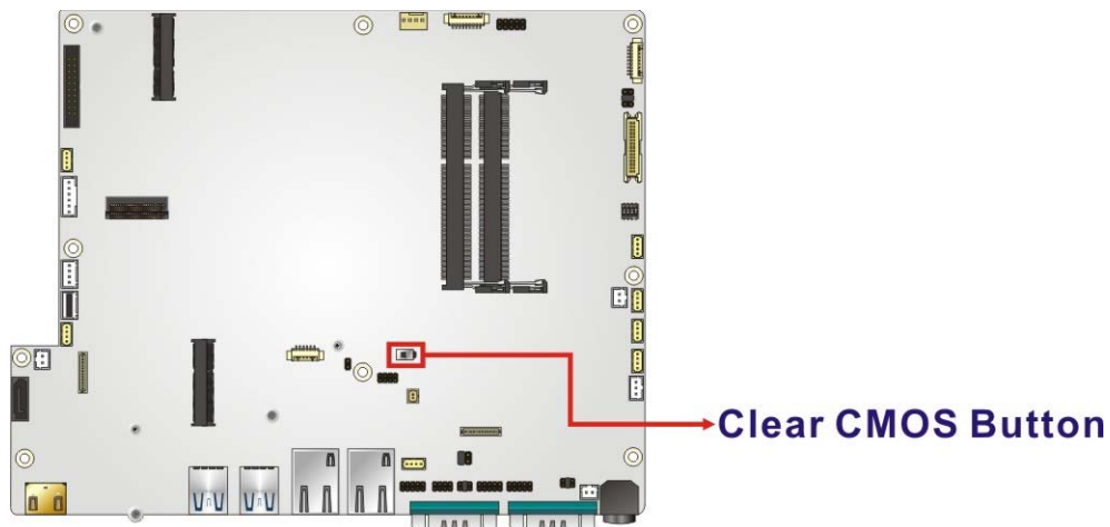
Figure 3-19: Clear CMOS Button Location
