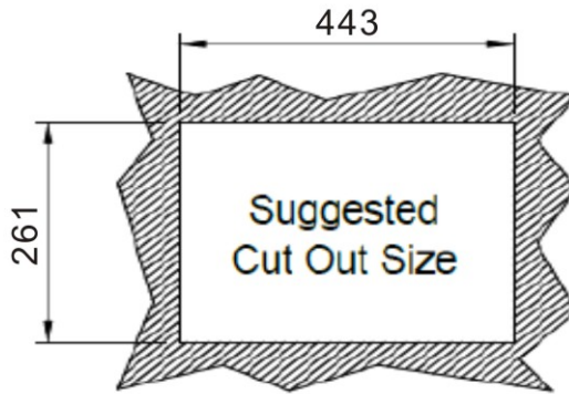
Figure 3-25: AFL3-W19C-ULT3 Cutout Dimensions
