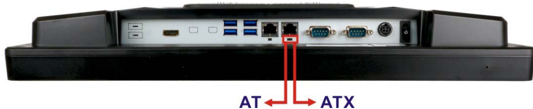
Figure 3-20: AT/ATX Switch Location
