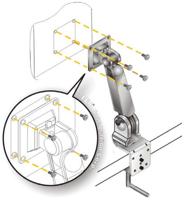
Figure 3-32: Arm Mounting
