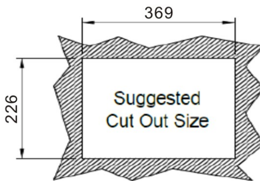
Figure 3-24: AFL3-W15C-ULT3 Cutout Dimensions
