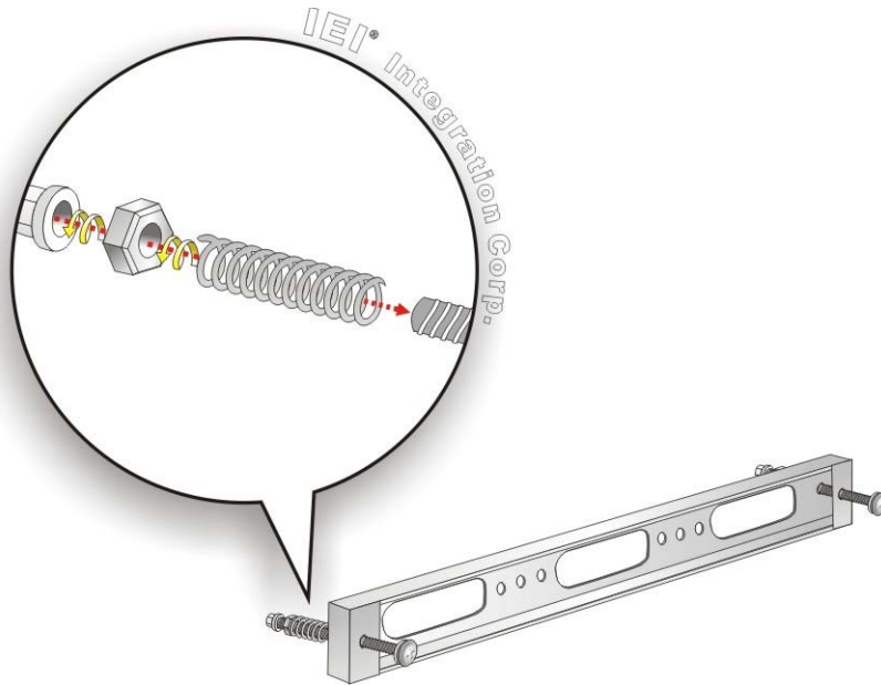
Figure 3-28: Rack Mounting Kit Installation
