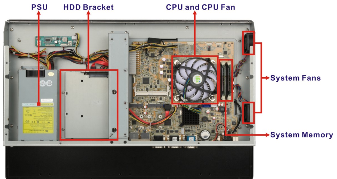
Figure 1-6: PPC-F22A-H81 Internal Components
