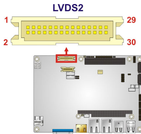
Figure 3-12: LVDS2 Connector Location
