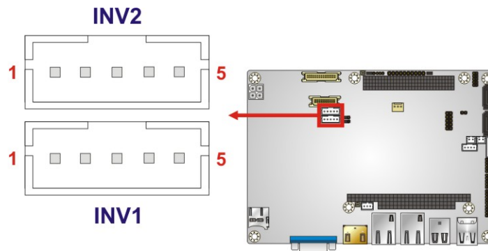
Figure 3-4: Backlight Inverter Connector Locations
