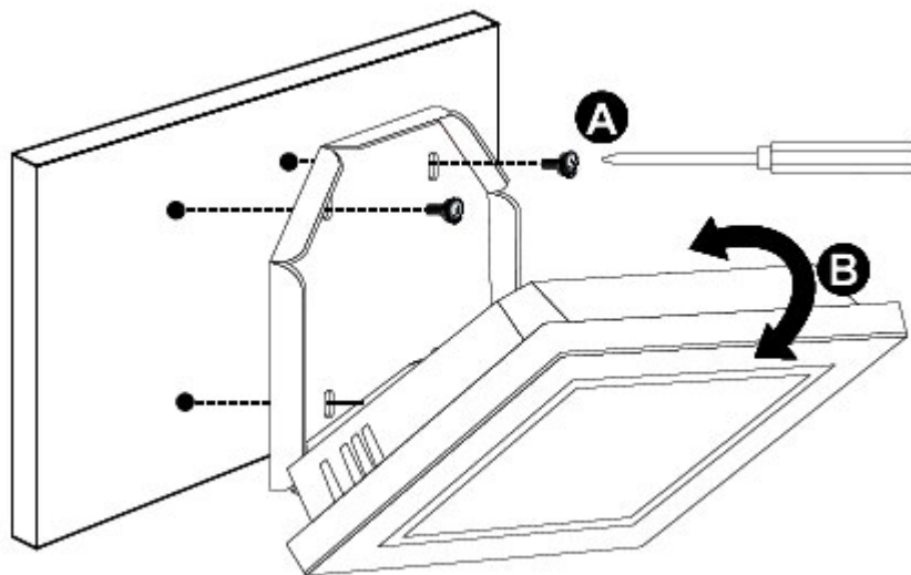
Figure 3-24: Secure V-Stand to Mounting Area
