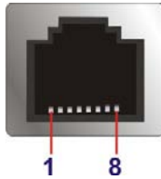
Figure 3-26: RJ-45 RS-422/485 Serial Port Pinout Location
