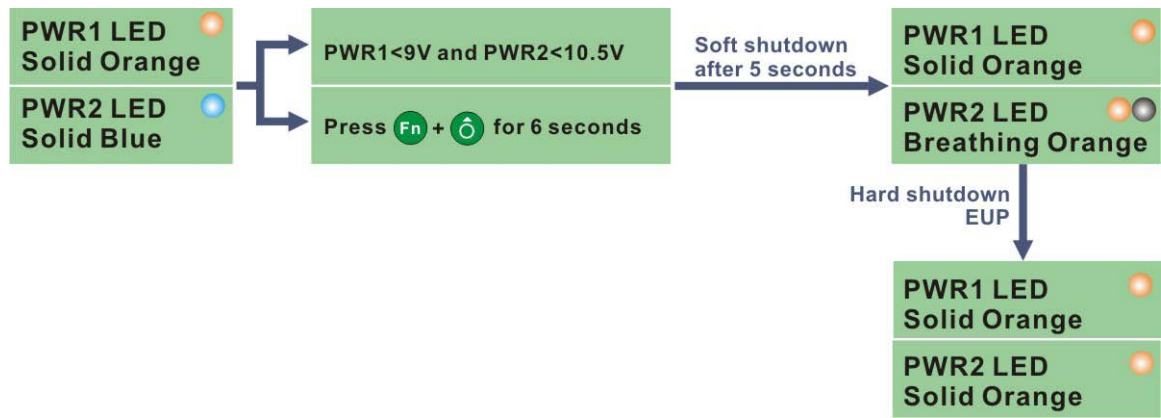
Figure 3-40: ACC Off: Shutdown
