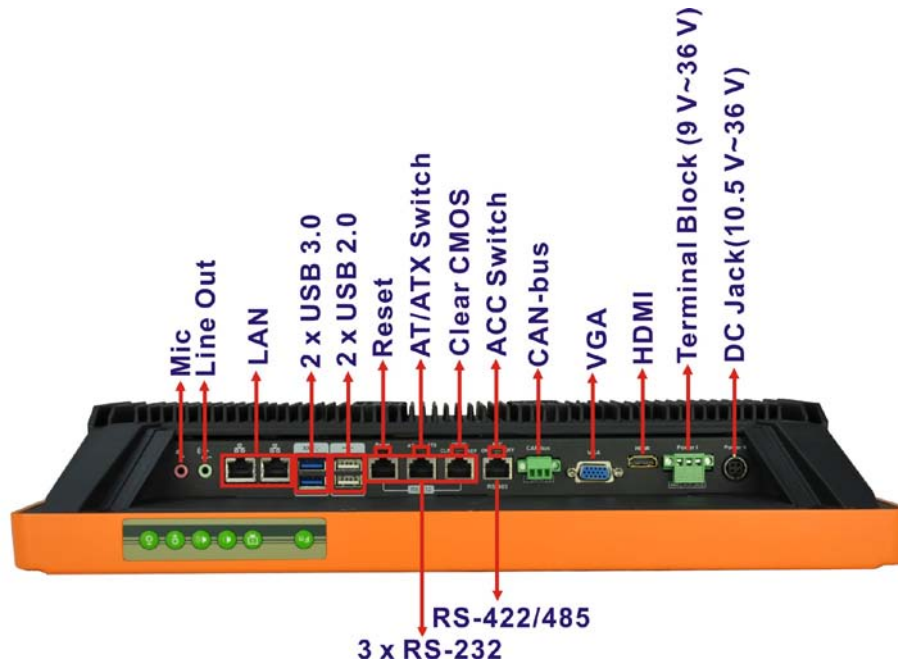
Figure 1-4: Bottom View
