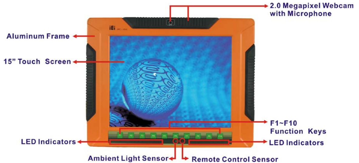
Figure 1-2: Front View
