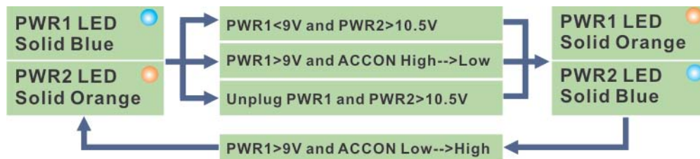
Figure 3-35: ACC On: Switch Between PWR1 and PWR2
