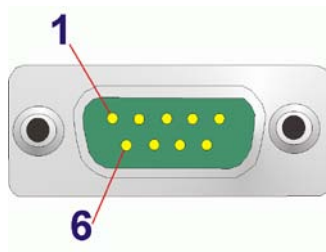
Figure 3-24: DB-9 Connector Pinout Location
