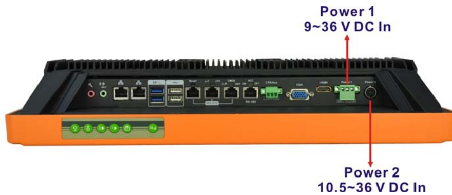
Figure 3-32: Power Connectors
