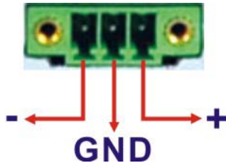
Figure 3-17: CAN-bus Terminal Block Pinouts
