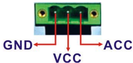
Figure 3-21: 3-pin Terminal Block Pinouts
