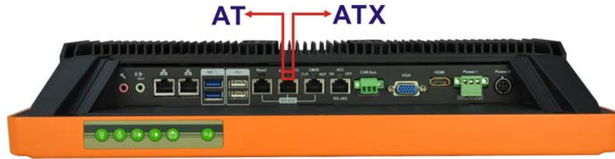
Figure 3-16: AT/ATX Power Mode Switch
