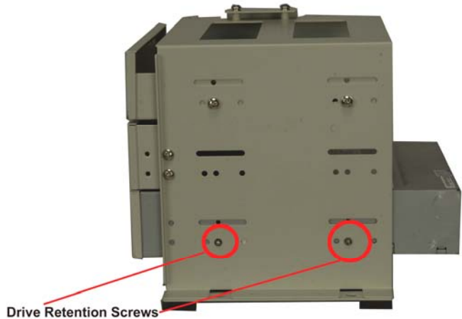
Figure 14: Install 5.25" Optical Drive Retention Screws
