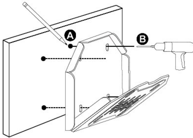
Figure 3-20: Drill Pilot Holes for V-Stand
