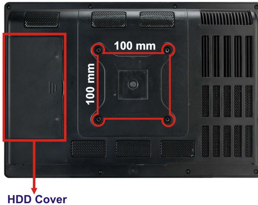
Figure 1-7: Rear View
