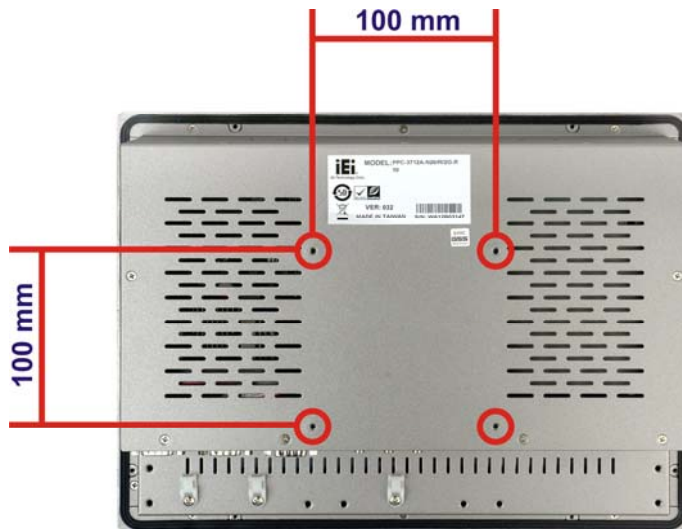
Figure 3-38: Stand Mounting Retention Screw Holes
