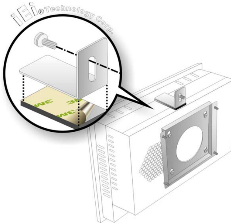
Figure 3-25: Secure the Chassis
