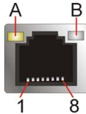
Figure 3-40: RJ-45 LAN Connector
