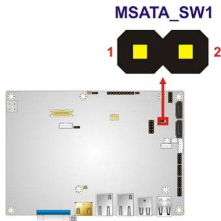
Figure 3-6: mSATA/PCIe Mini Mode Selection Jumper Location
