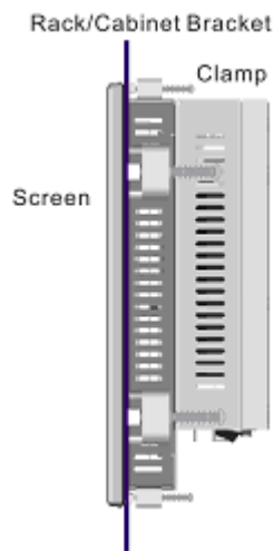
Figure 3-33: Securing the PPC-3708A-N26 Rack/Cabinet Bracket
