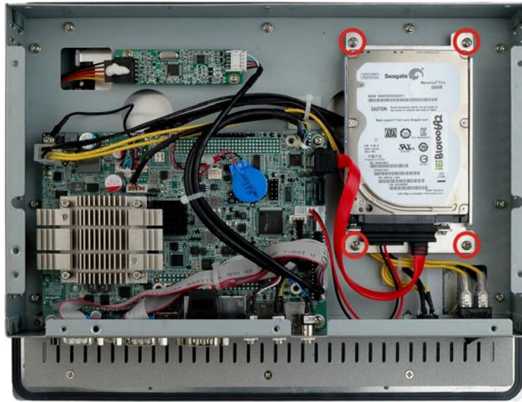
Figure 3-17: Replacing the PPC-3710A-N26 HDD Bracket
