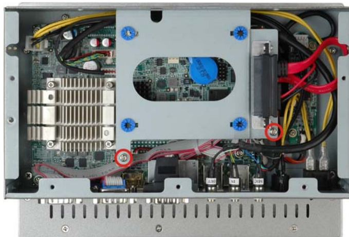
Figure 3-12: PPC-3708A-N26 HDD Bracket Retention Screws (Inside)
