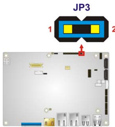
Figure 3-4: AT/ATX Power Selection Jumper Location
