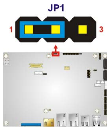
Figure 3-5: Clear CMOS Jumper Location
