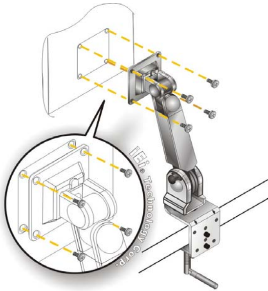
Figure 3-37: Arm Mounting
