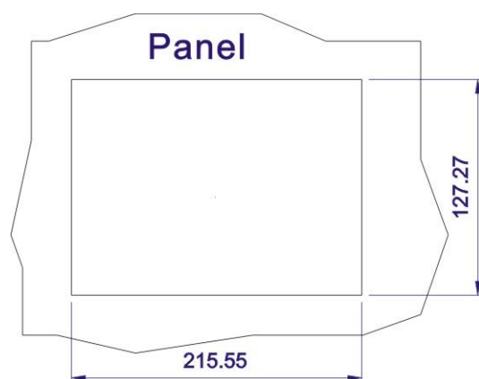
Figure 4-15: AFL-07A-N270 Panel Opening
