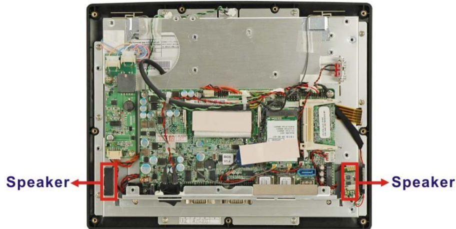
Figure 2-11: Stereo Speakers
