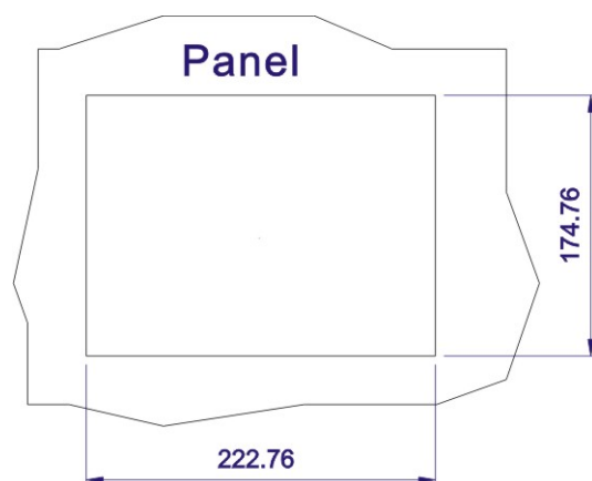
Figure 4-16: AFL-08AH-N270 Panel Opening
