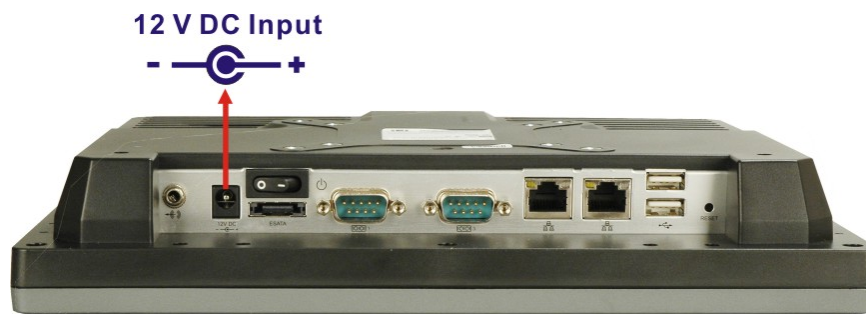
Figure 2-12: Power Connector
