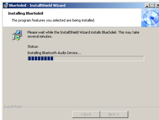
Figure 7-40: Installing BlueSoleil
