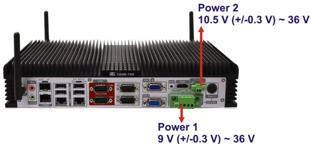
Figure 3-35: Power Connectors
