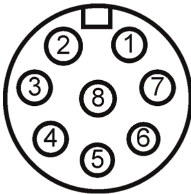
Figure 3-7: Serial Port
