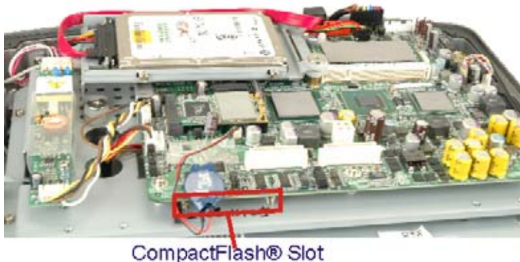
Figure 3-4: CompactFlash® Install
