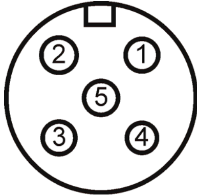
Figure 3-8: CAN & Audio Port
