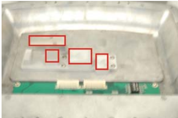
Figure 6-4: Thermal Pads
