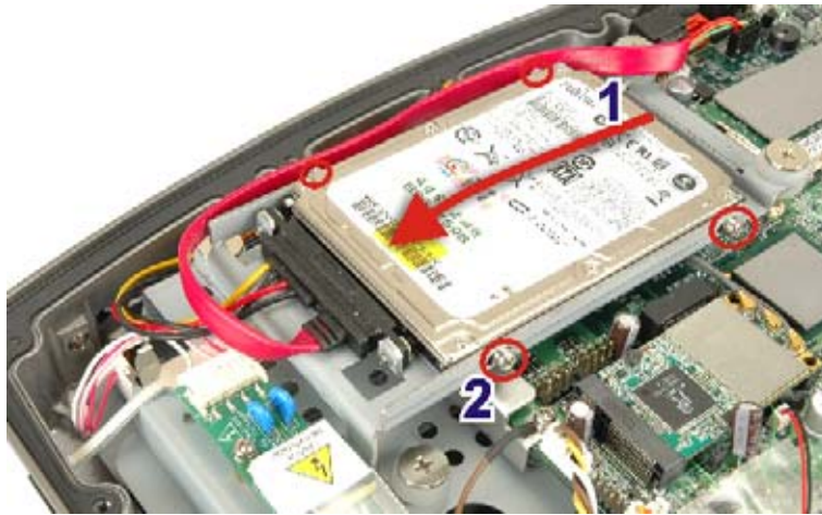
Figure 3-3: HDD Installation
