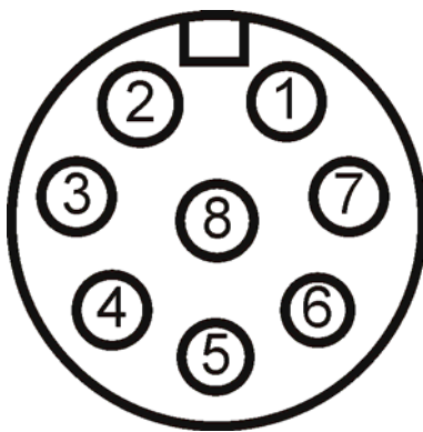
Figure 3-6: LAN Port
