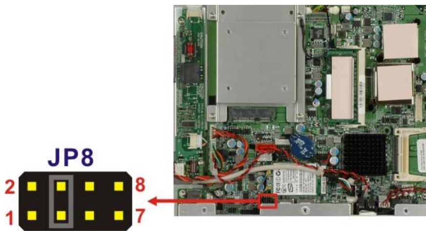
Figure 4-9: COM3 RX Function Select Jumper Location
