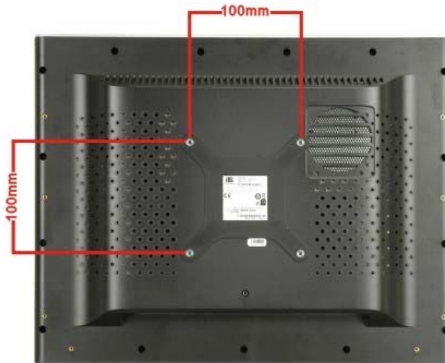
Figure 1-3: AFL-15A-N270 Rear View
