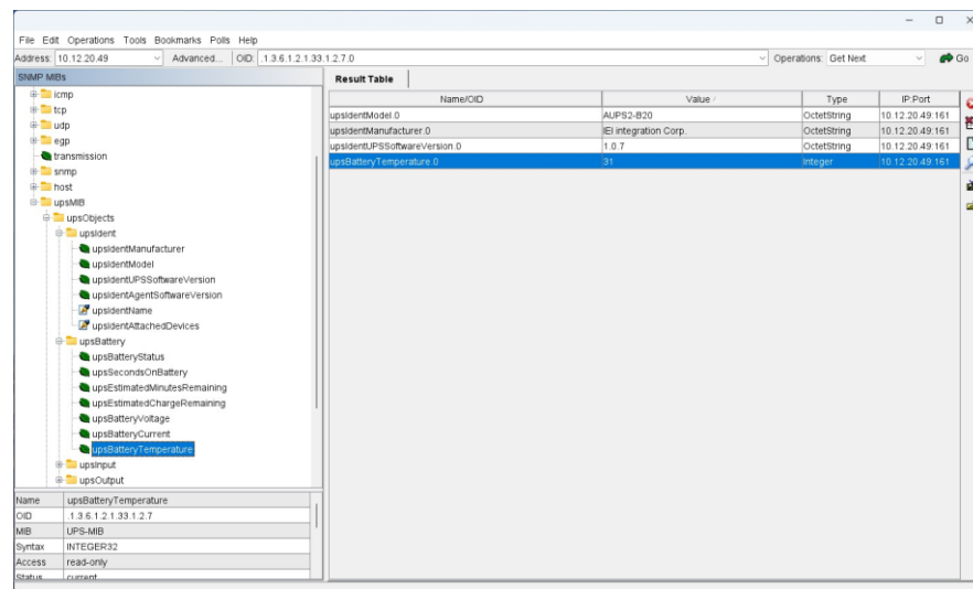
Figure 4-21: Remote Monitoring screen diagram
