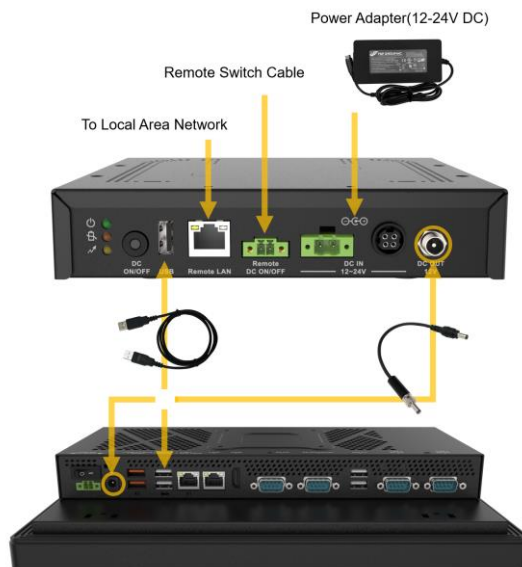
Figure 3-8: AUPS2-B20 Series and Panel PC Connection
