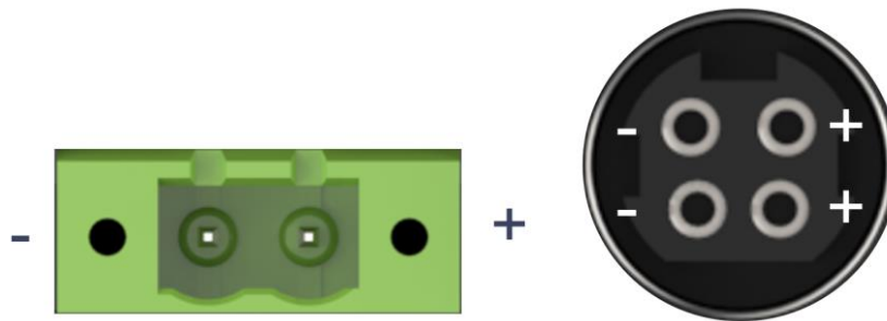
Figure 3-11: Power Input Connector
