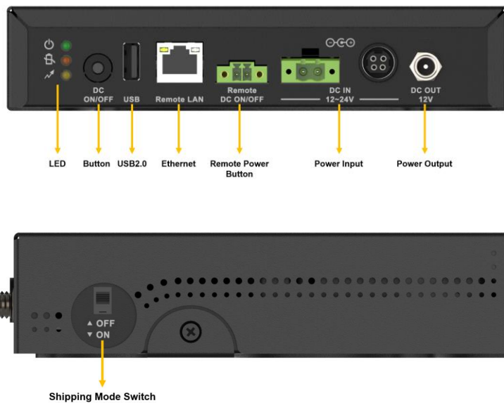
Figure 3-9: External Peripheral Interface Connectors
