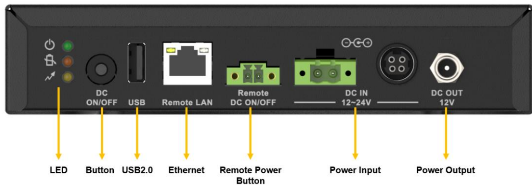
Figure 1-2: AUPS2-B20 Series I/O Interface Panel (1/2)
