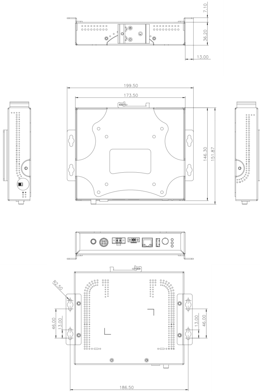
Figure 1-5: AUPS2-B20 Dimensions (mm)
