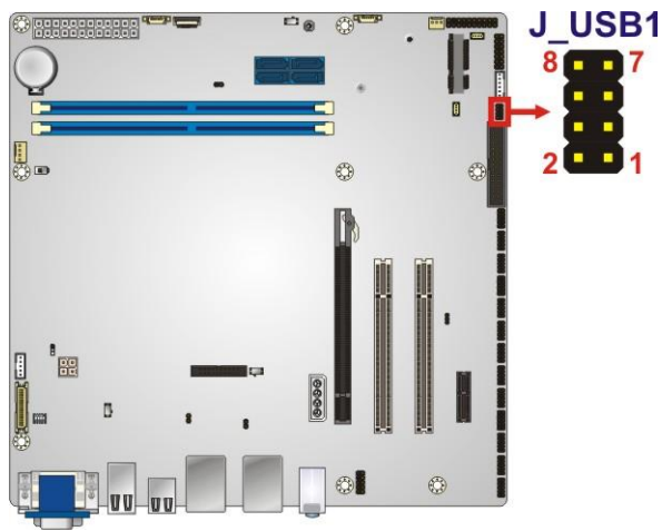
Figure 3-33: USB 2.0 Connector Locations
