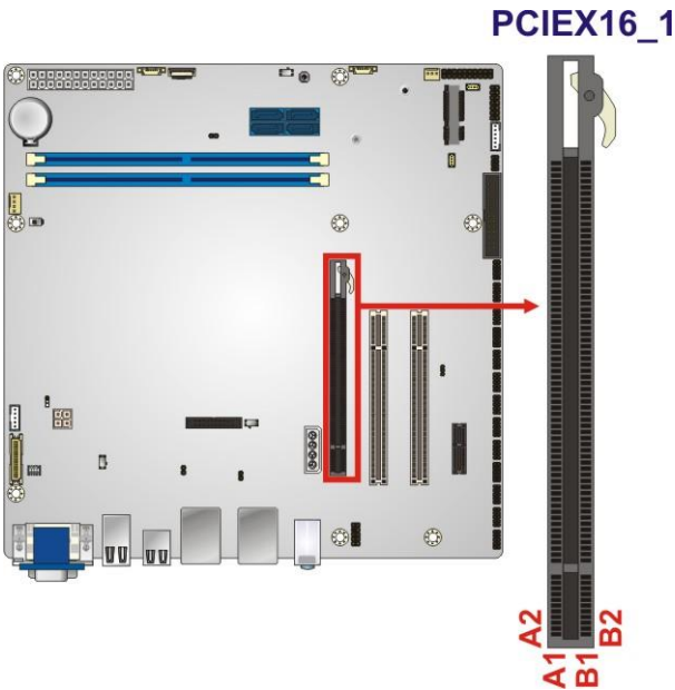
Figure 3-23: PCIe x16 Slot Location
