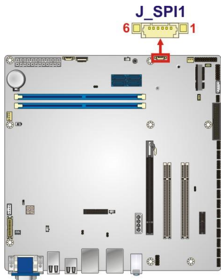
Figure 3-30: SPI Flash Connector Location
