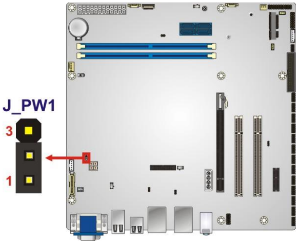
Figure 4-19: LVDS Voltage Selection Jumper Location
