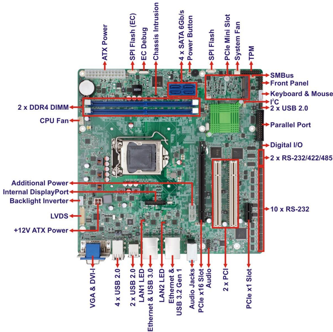
Figure 1-2: Connectors
