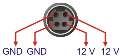
Figure 3-32: Power Connector (4-pin DIN)
