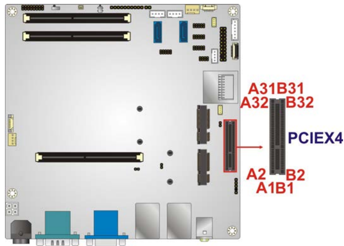
Figure 3-16: PCIe x4 Slot Location
