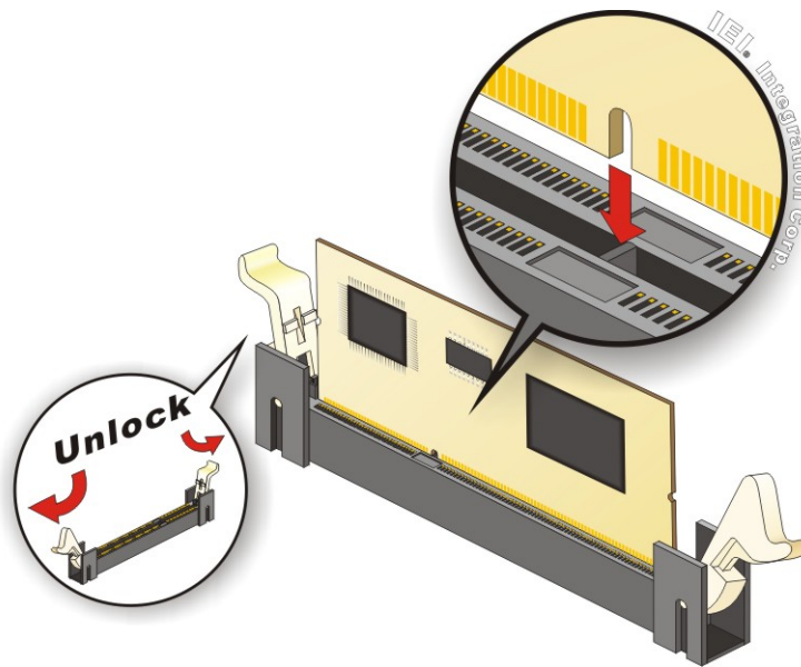
Figure 4-2: IPMI Module Installation
