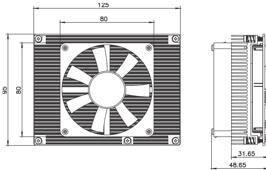
Figure 1-4: ICE-BDE-T7 Dimensions (with heatsink) (mm)
