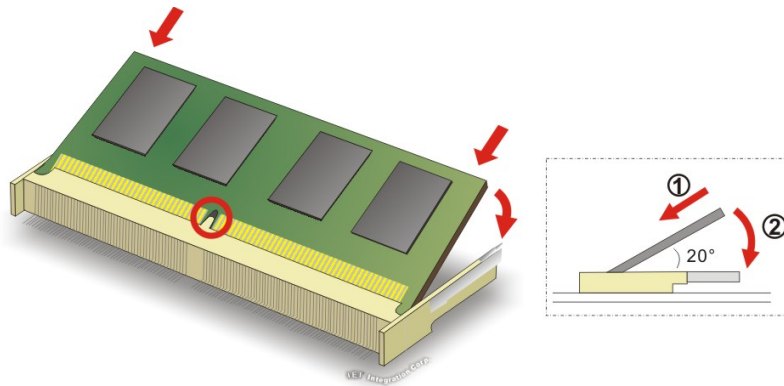
Figure 4-1: SO-DIMM Installation
