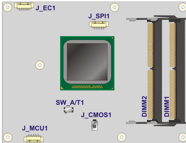
Figure 3-1: Connectors (Front Side)
