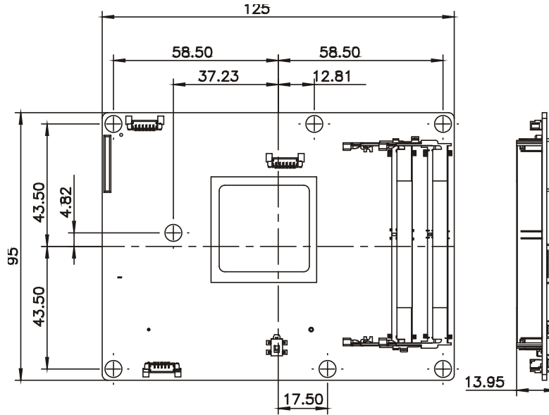
Figure 1-3: ICE-BDE-T7 Dimensions (without heatsink) (mm)
