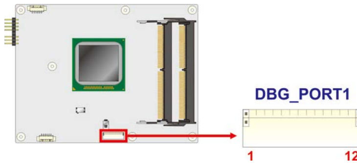
Figure 3-7: LPC Debug Port Location
