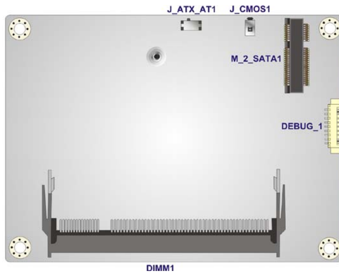
Figure 3-2: Connector and Jumper Locations (Rear)
