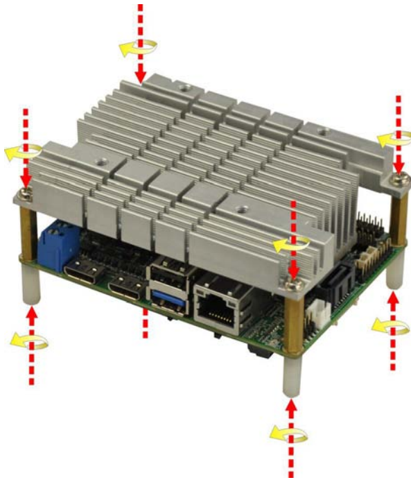
Figure 4-4: Heat Sink Retention Screws
