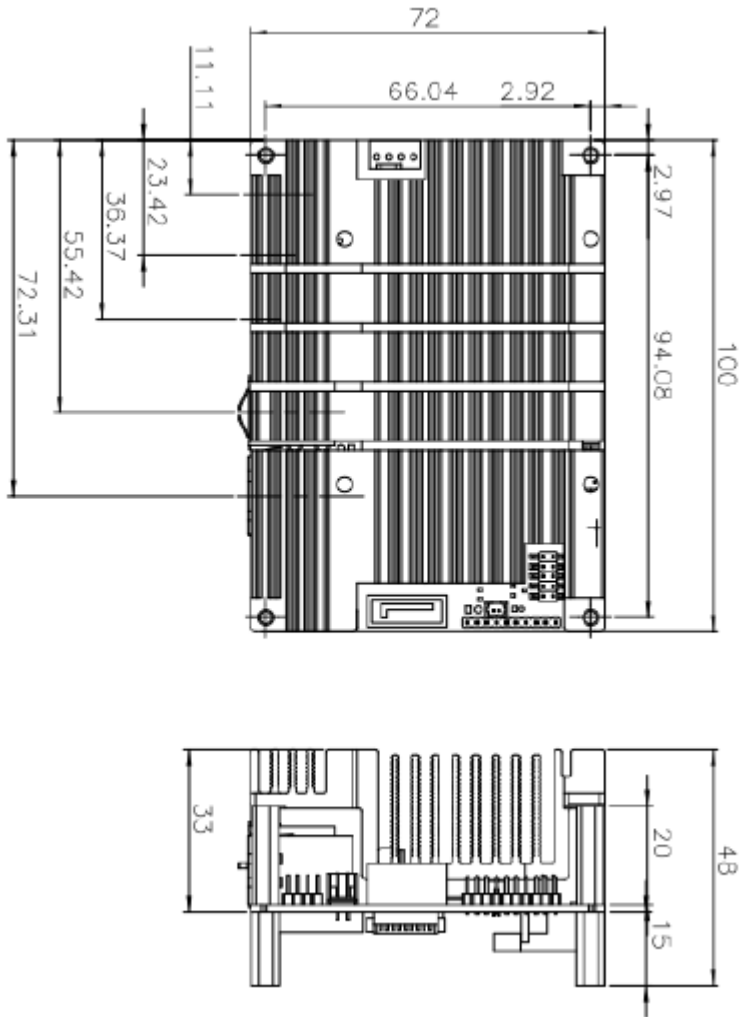
Figure 1-4: Dimensions (mm)
