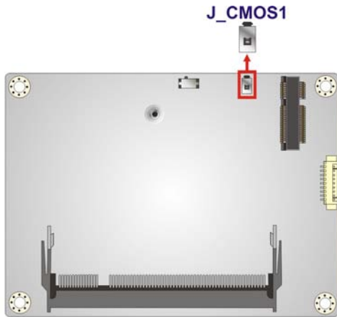
Figure 3-8: Clear CMOS Button Location
