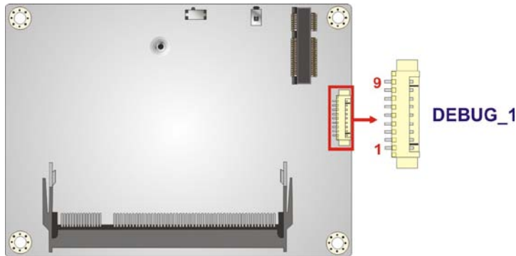
Figure 3-11: Debug Port Connector Location
