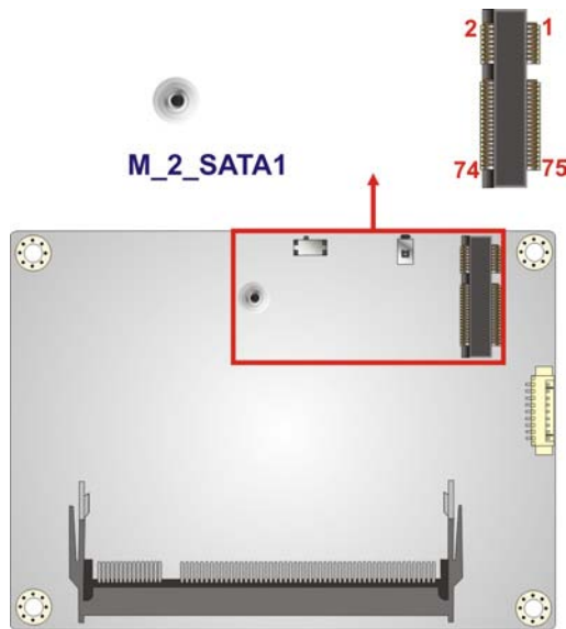
Figure 3-15: M.2 2242 (B key) Socket Location
