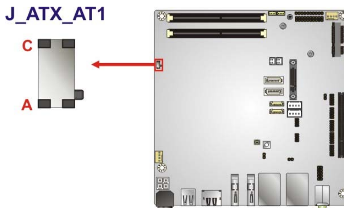
Figure 4-9: AT/ATX Mode Select Switch Location
