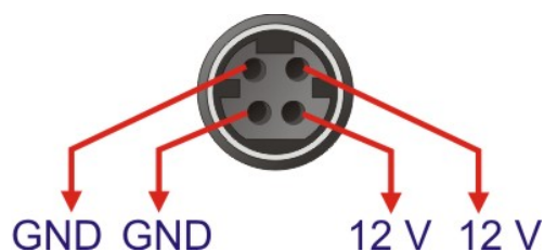
Figure 3-31: Power Connector
