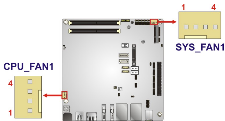
Figure 3-9: Fan Connector Locations
