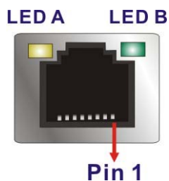
Figure 3-30: Ethernet Connector
