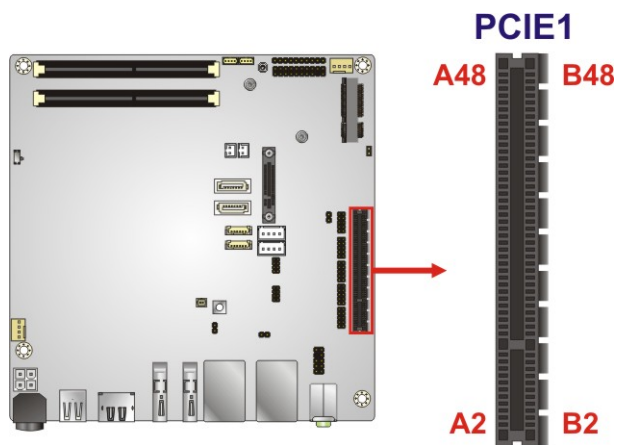
Figure 3-16: PCIe x1 Slot Location
