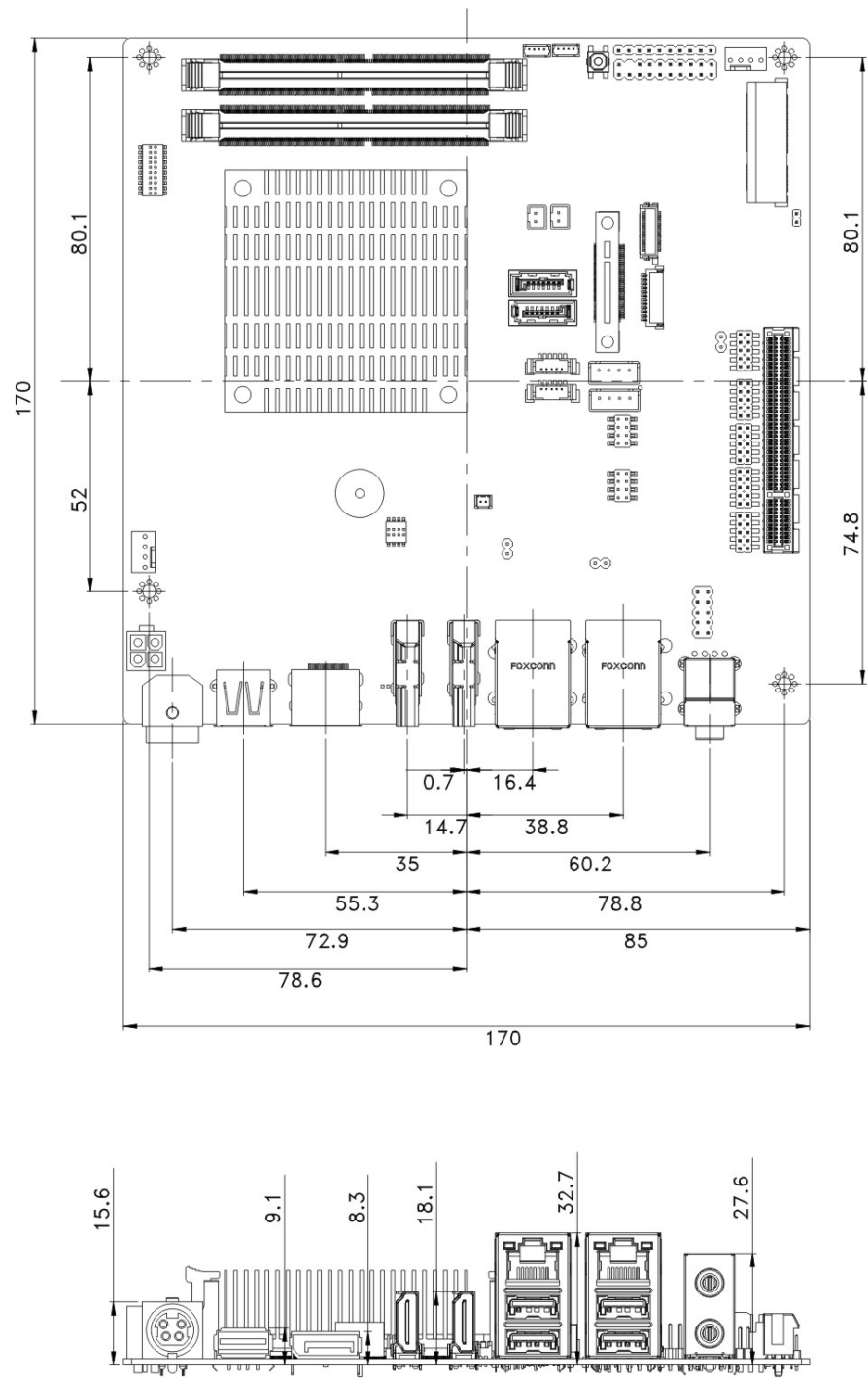
Figure 1-4: Dimensions (mm)
