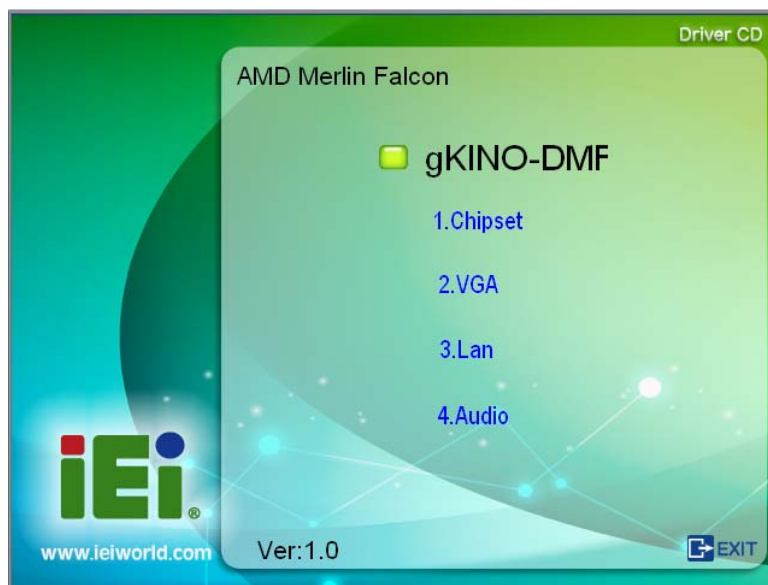
Figure 6-1: Available Drivers
