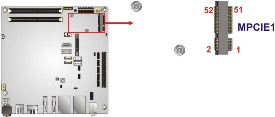
Figure 3-15: PCIe Mini Card Slot Location
