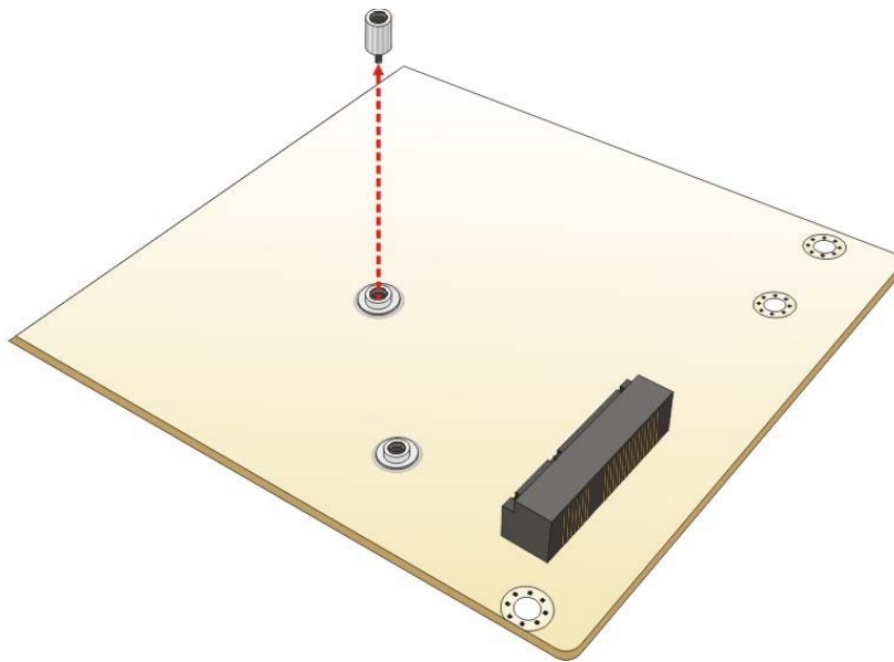
Figure 4-5: Removing Retention Screw and Standoff
