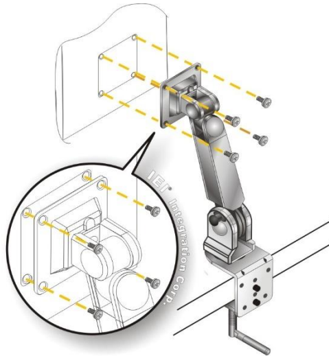
Figure 3-10: Arm Mounting
