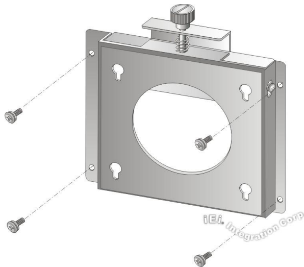
Figure 3-6: Wall-mounting Bracket
