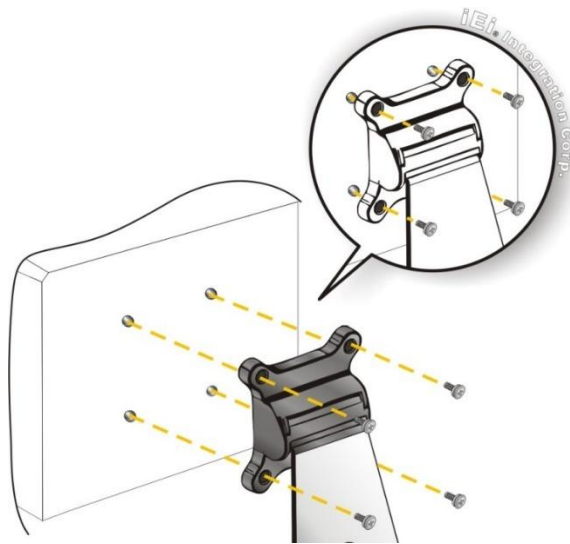
Figure 3-11: Stand Mounting (Stand-Cxx)
