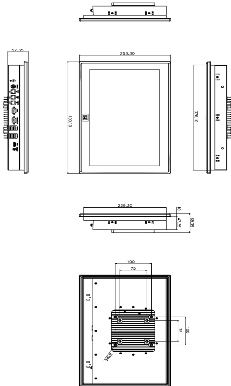
Figure 1-5: PPC2-CW156A-ADLP Dimensions (mm)
