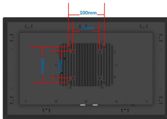
Figure 3-9: Arm Mounting Retention Screw Holes
