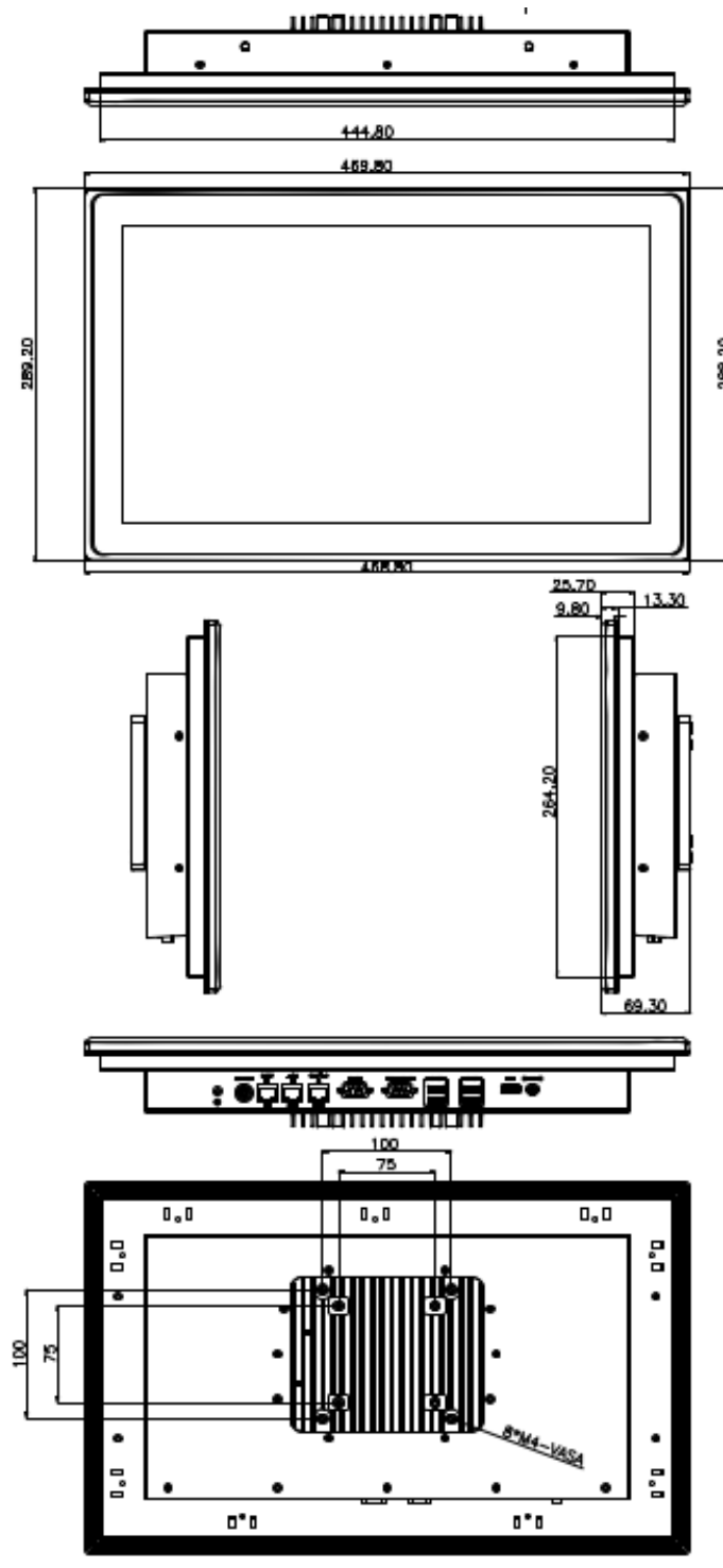
Figure 1-6: PPC2-CW185A-ADLP Dimensions (mm)
