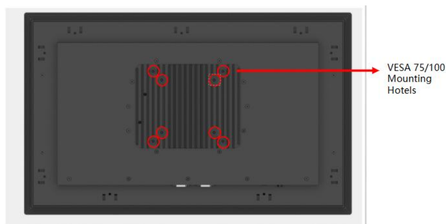
Figure 1-3: Rear View
