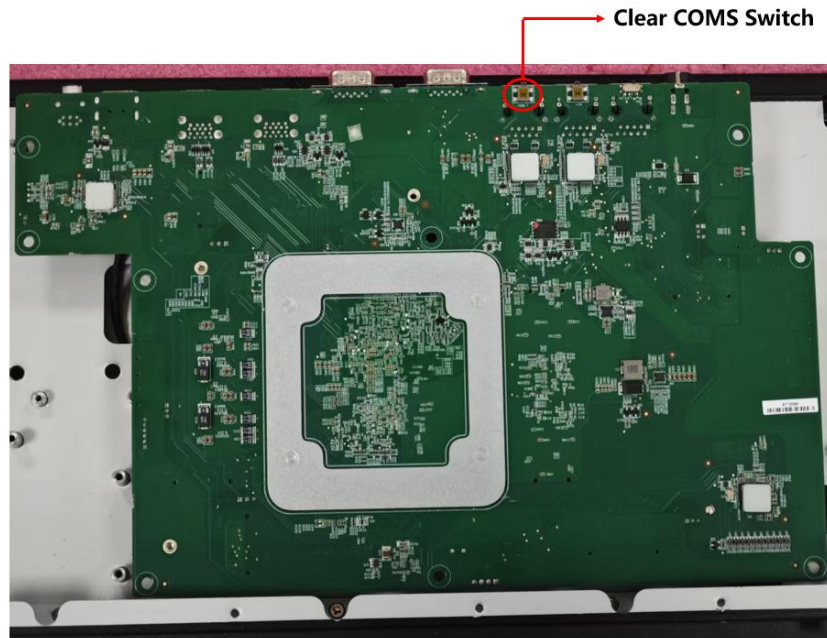
Figure 3-4: Clear CMOS Button Location
