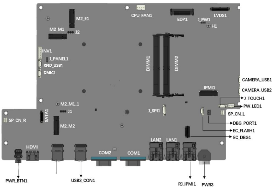
Figure 6-1: Main Board Layout Diagram
