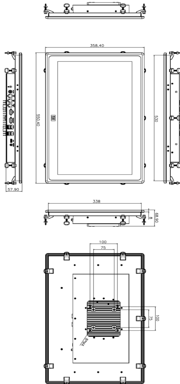
Figure 1-7: PPC2-CW215A-ADLP Dimensions (mm)
