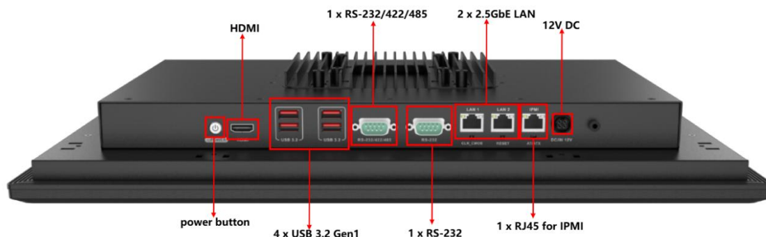
Figure 1-4: PPC2-CWxxxA-ADLP Series Bottom Panel
