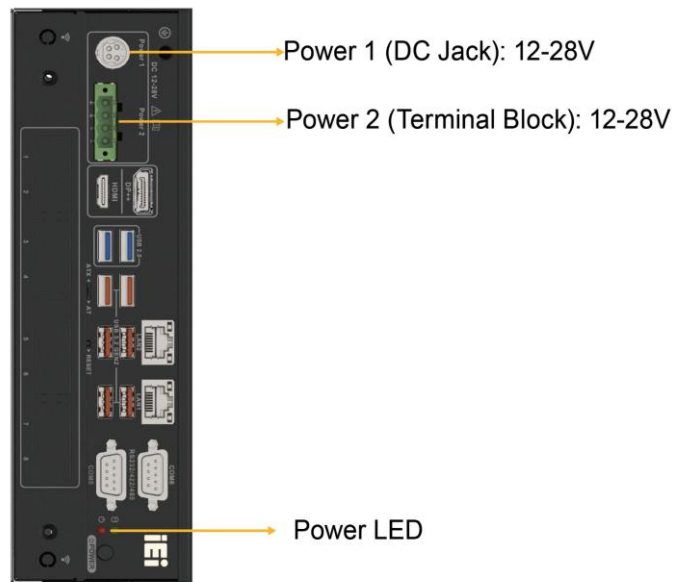
Figure 3-23: Power Connectors
