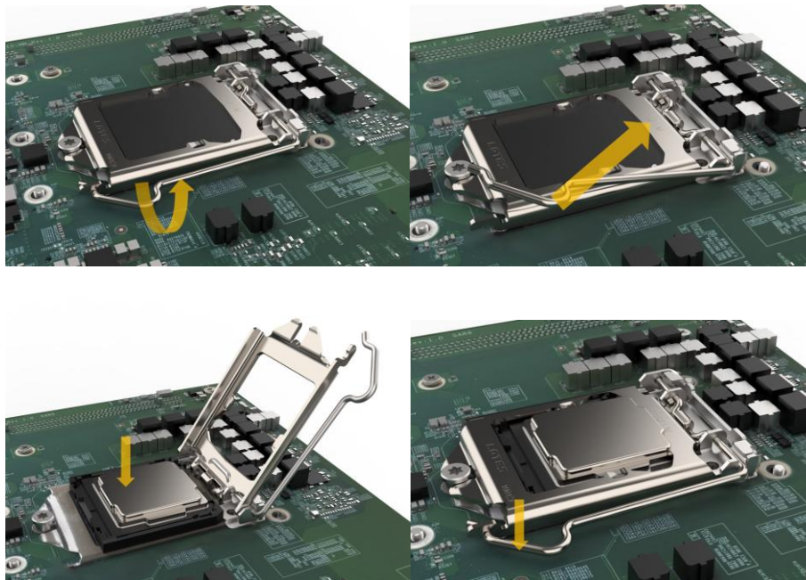
Figure 3-3: CPU Installation
