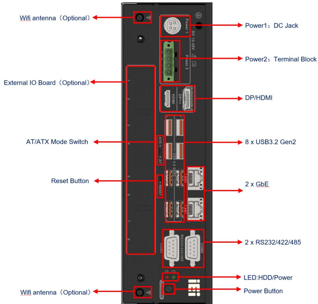
Figure 1-2: Front Panel
