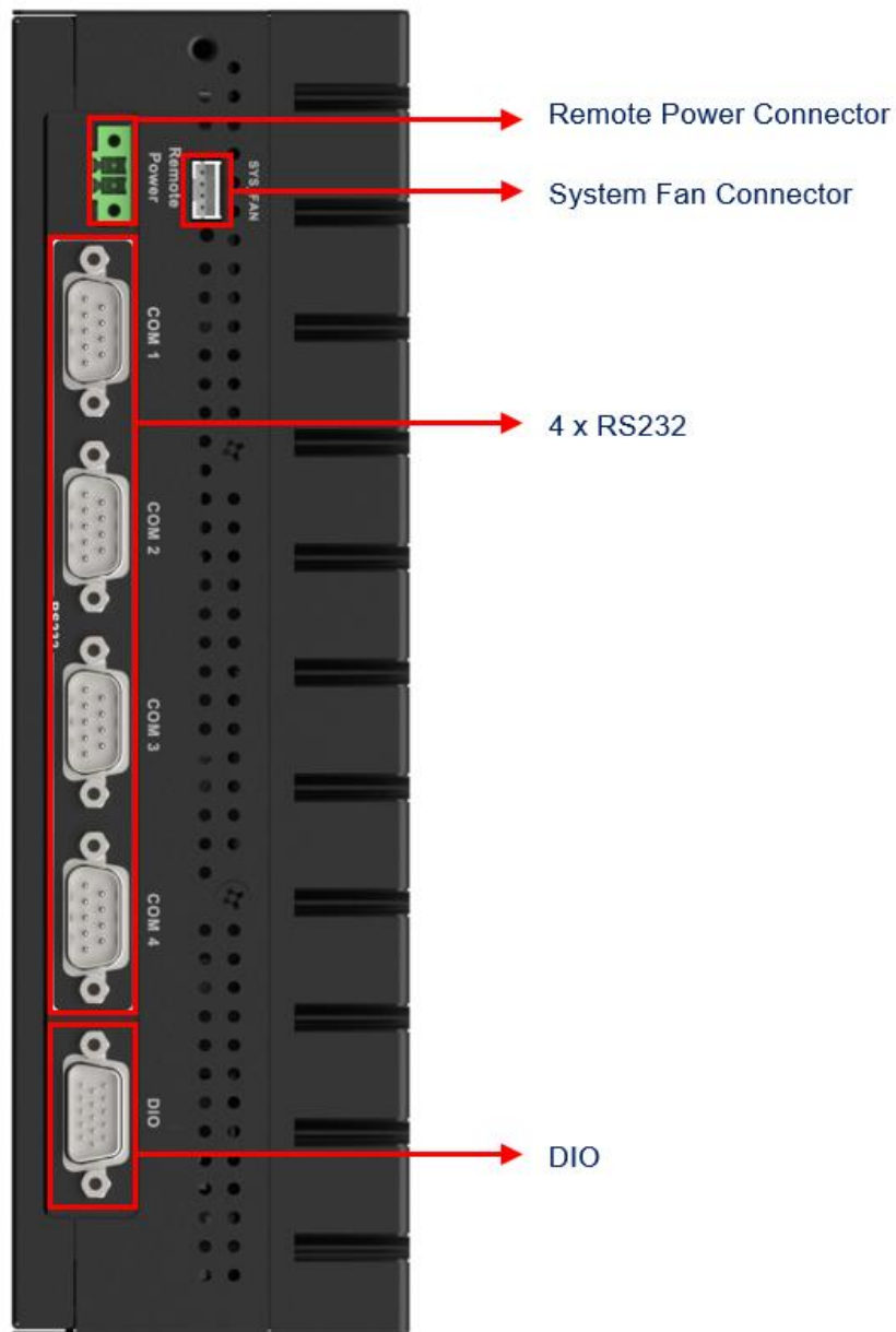
Figure 1-3: Rear Panel
