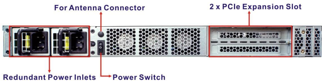
Figure 1-3: PUZZLE-IN001 Rear Panel
