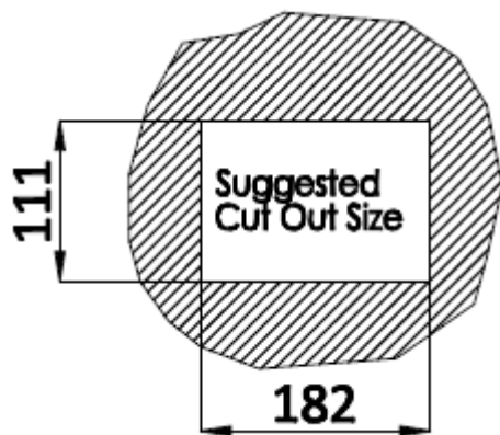
Figure 3-9: Cutout Dimensions
