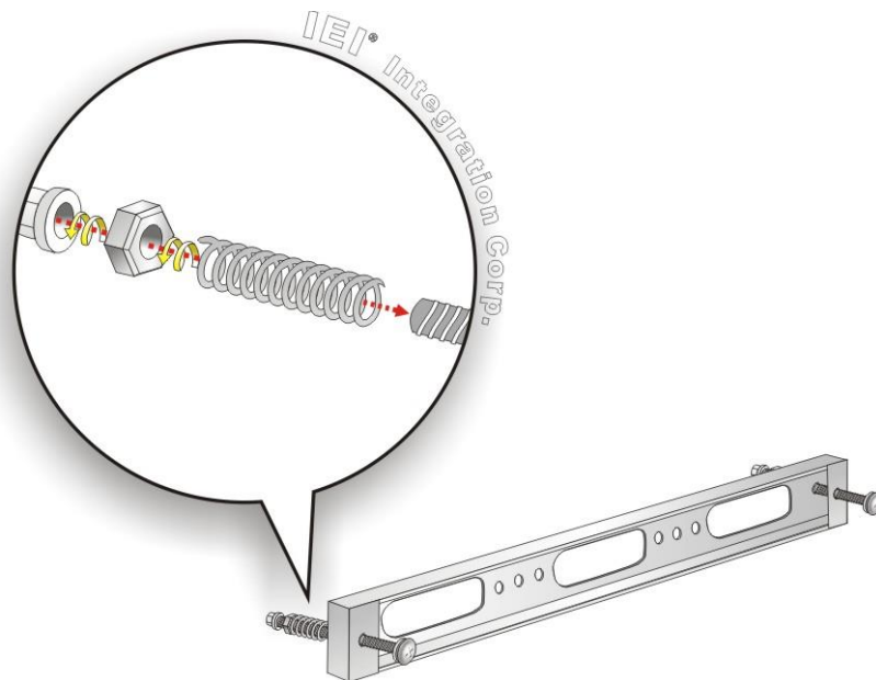
Figure 3-10: Panel Mounting Kit Installation
