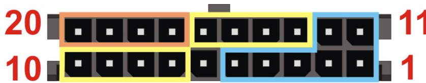
Figure 3-4: IO 1 Connector Pinout Locations
