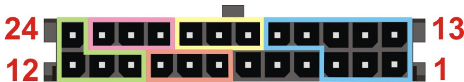
Figure 3-5: IO 2 Connector Pinout Locations
