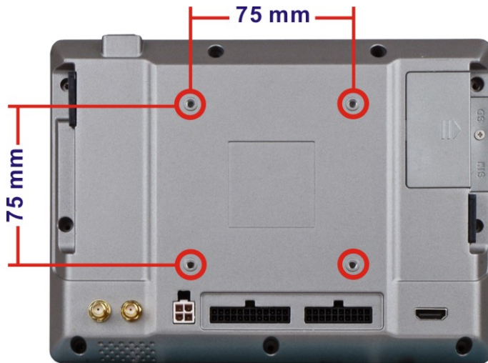
Figure 3-3: VESA Mount Retention Screw Holes
