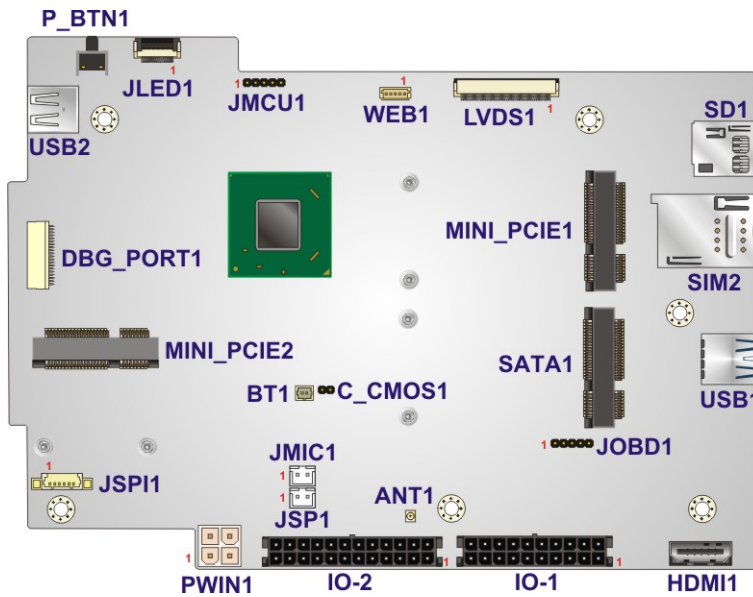
Figure 5-1: Main Board Layout Diagram (Front Side)
