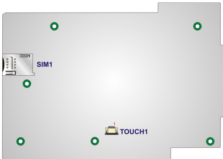
Figure 5-2: Main Board Layout Diagram (Solder Side)
