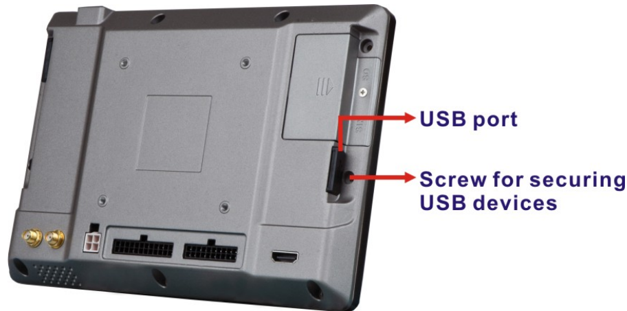
Figure 3-8: USB Connector
