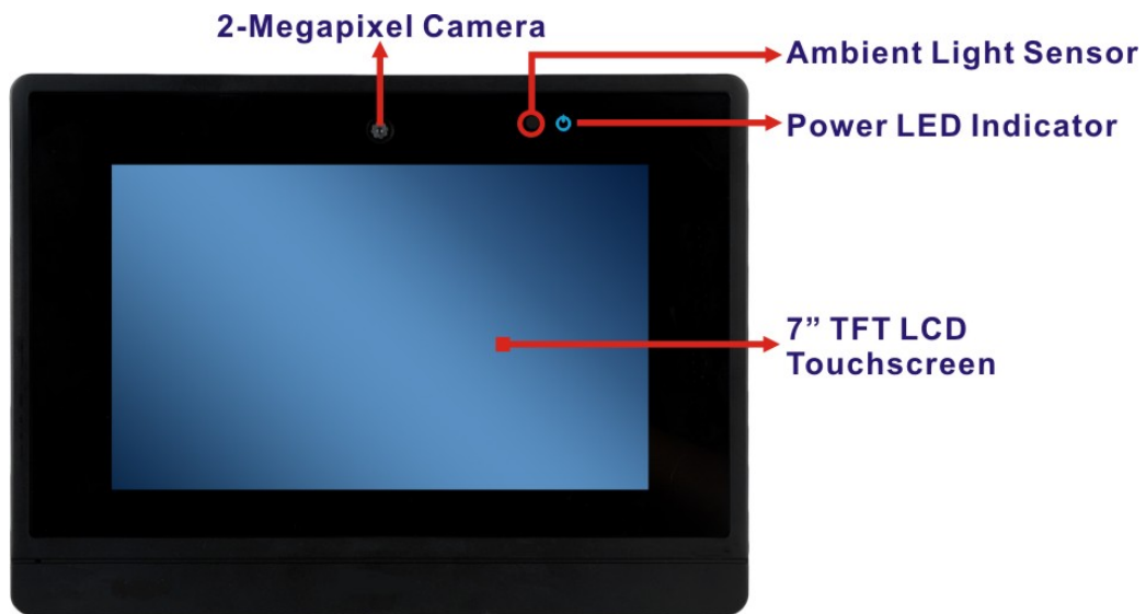
Figure 1-2: Front View
