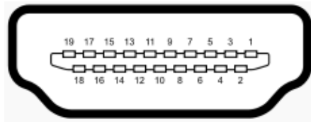
Figure 3-6: HDMI Connector
