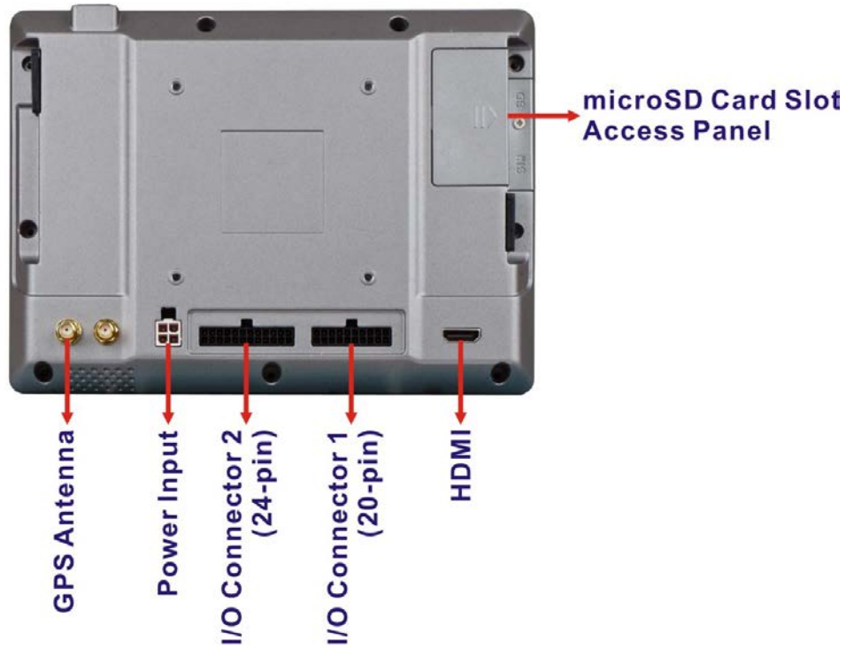
Figure 1-4: Rear Panel
