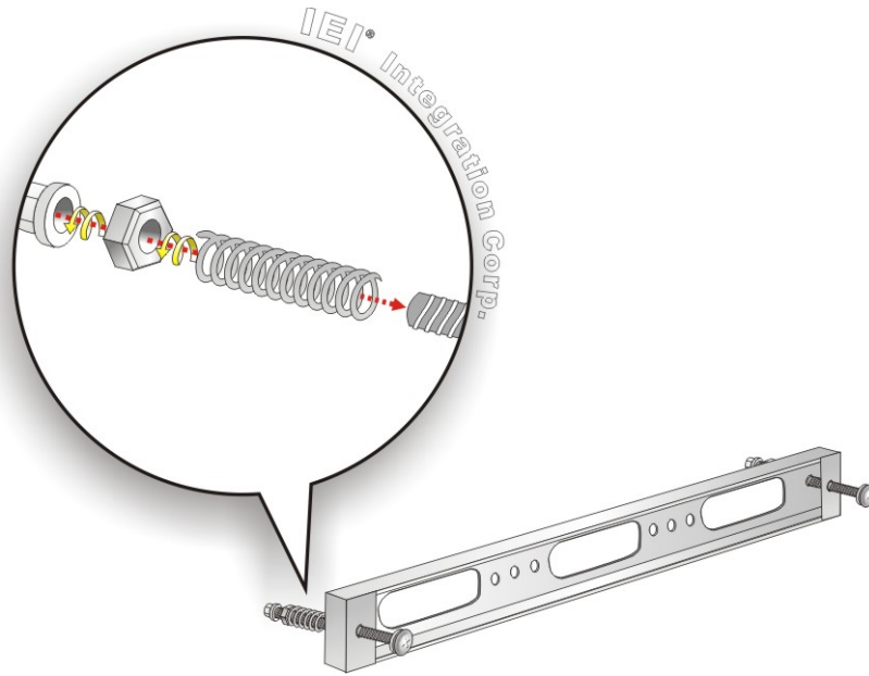
Figure 3-16: Rack Mounting Kit Installation
