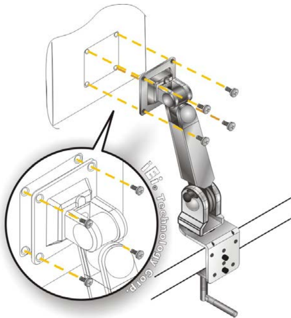
Figure 3-20: Arm Mounting
