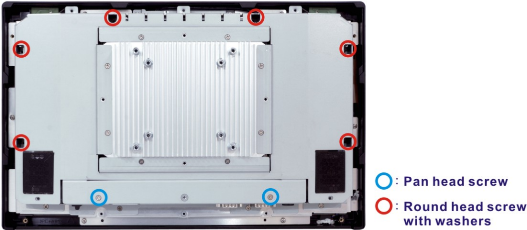
Figure 3-4: AFL3-W15C-ULT3 Aluminum Cover Retention Screws
