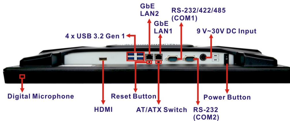
Figure 1-5: AFL3-W22C-ULT3 Bottom Panel
