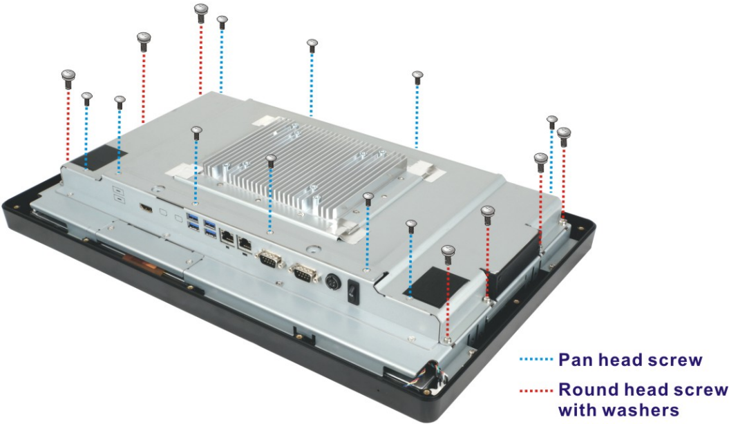
Figure 3-5: AFL3-W19C-ULT3 Aluminum Cover Retention Screws
