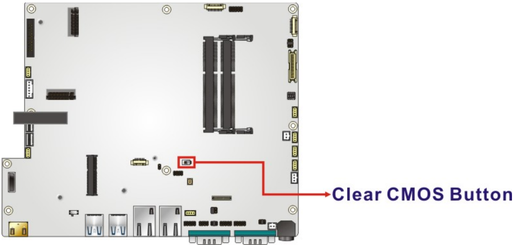
Figure 3-22: Clear CMOS Button Location
