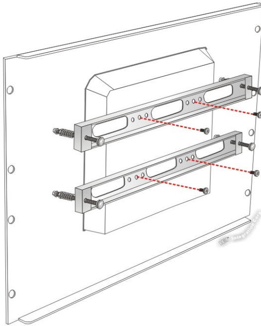
Figure 3-33: Securing Rack Mounting Brackets
