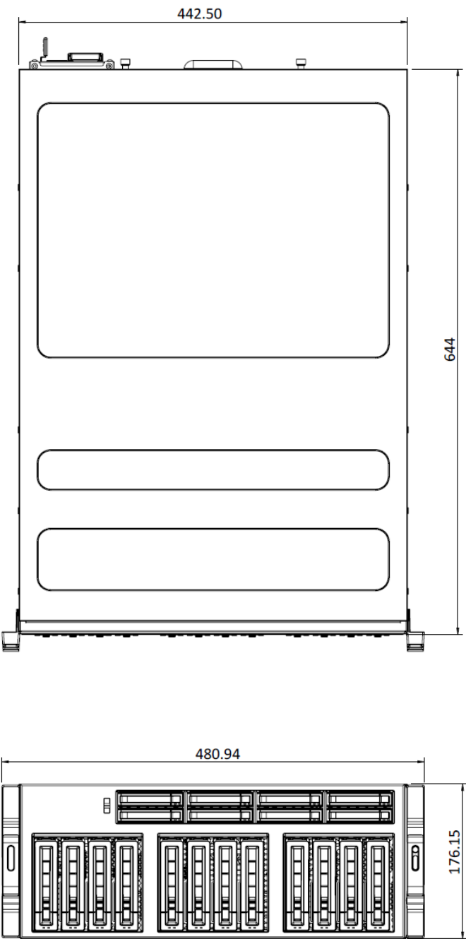
Figure 1-2: Dimensions (Unit: mm)
