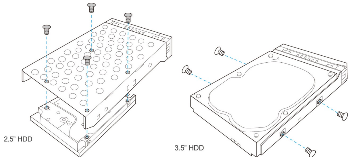
Figure 3-3: HDD Tray Installation (2.5\"/>
