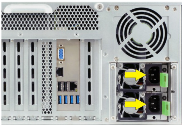
Figure 3-9: Power Connection
