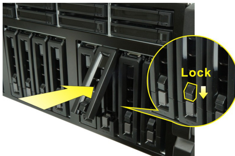
Figure 3-4: HDD Installation (2.5\"/>
