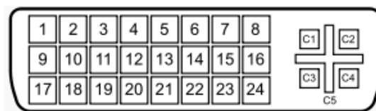
Figure 3-18: DVI-D Connector
