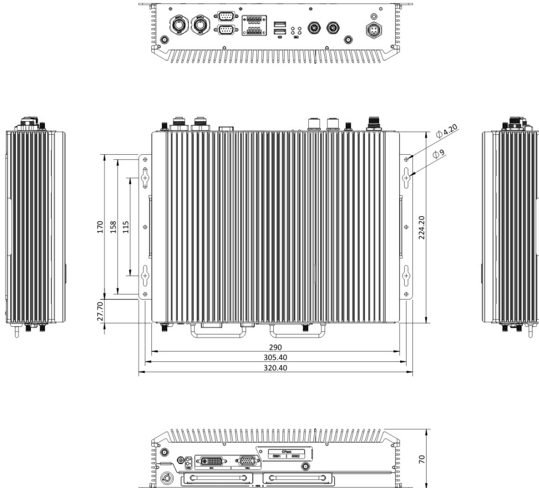
Figure 1-5: Dimensions (unit: mm)
