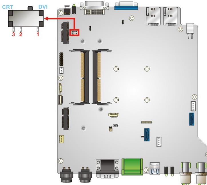
Figure 3-4: DVI/CRT Selection Switch Location
