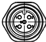
Figure 3-21: USB 2.0 Connector Pinout Location
