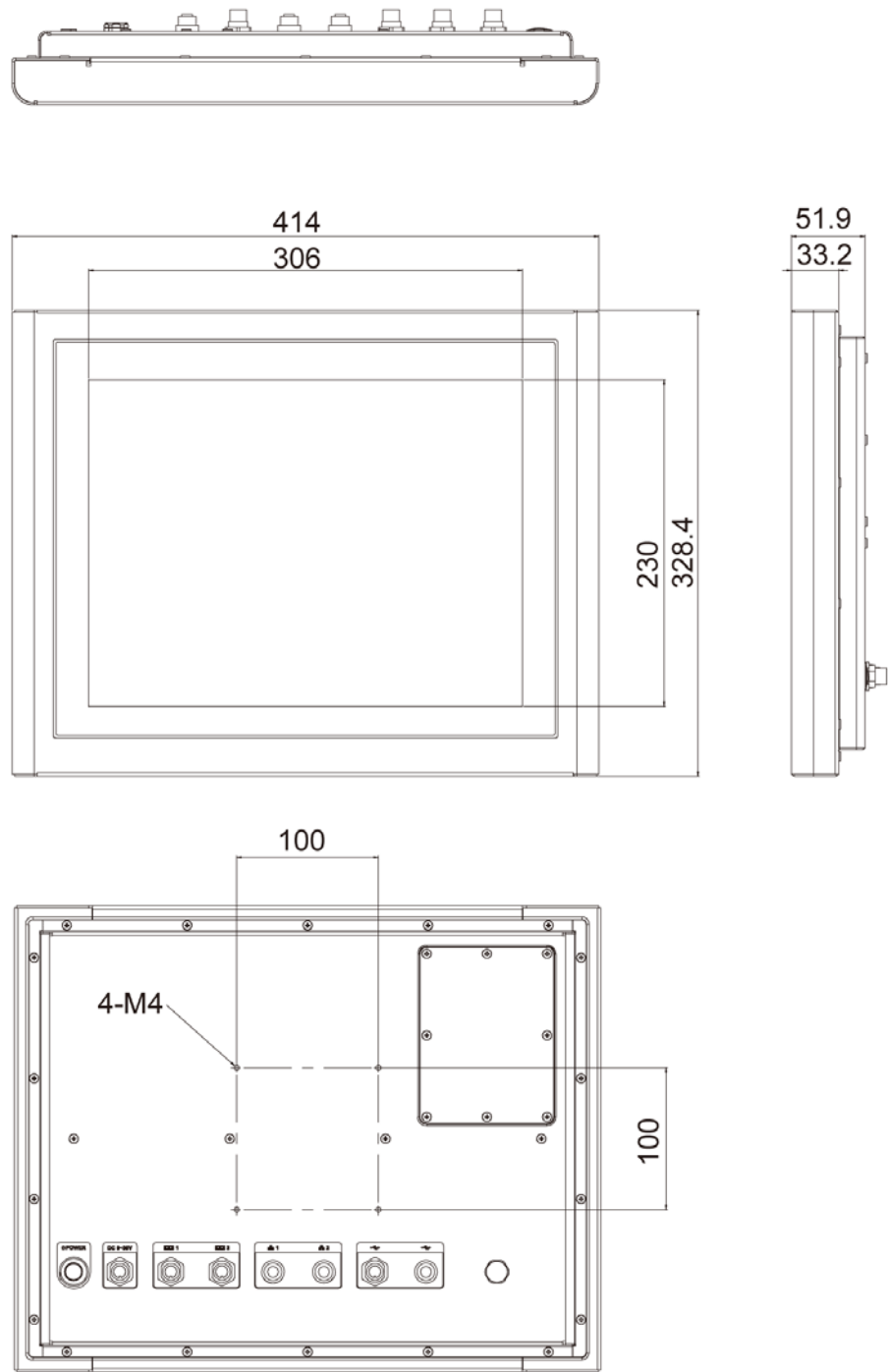
Figure 1-4: Dimensions (mm)
