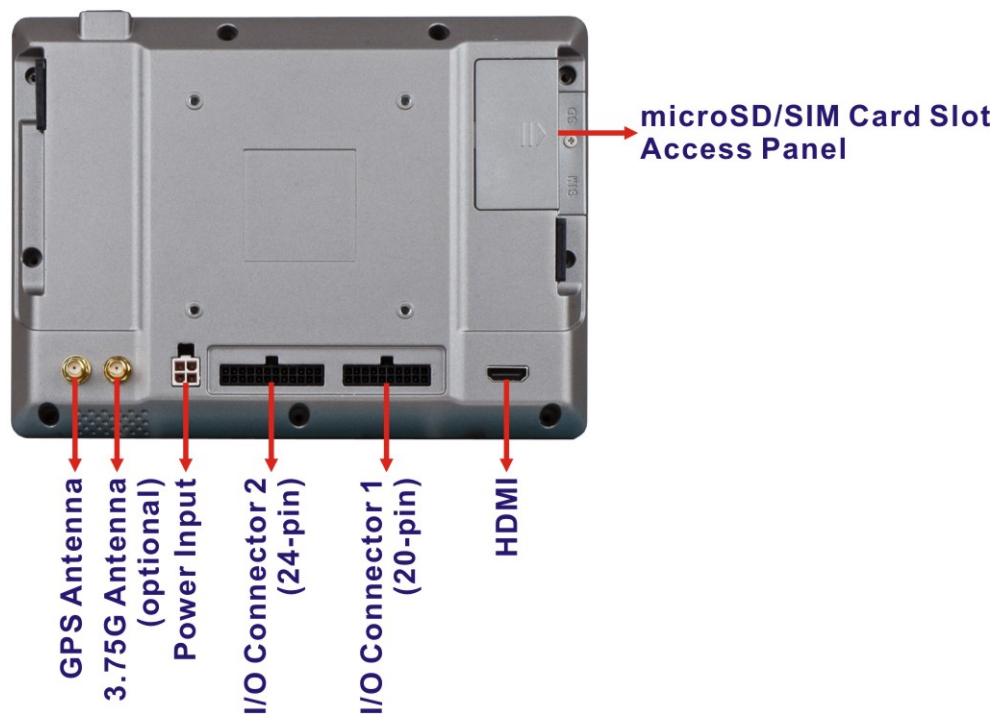
Figure 1-4: Rear Panel
