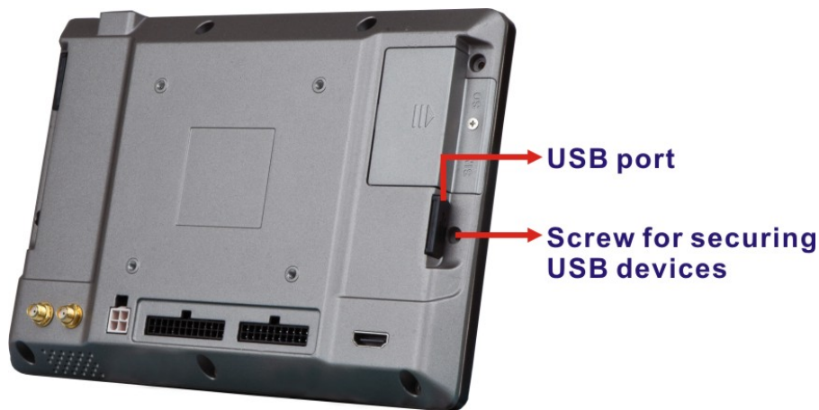
Figure 3-14: USB Connector
