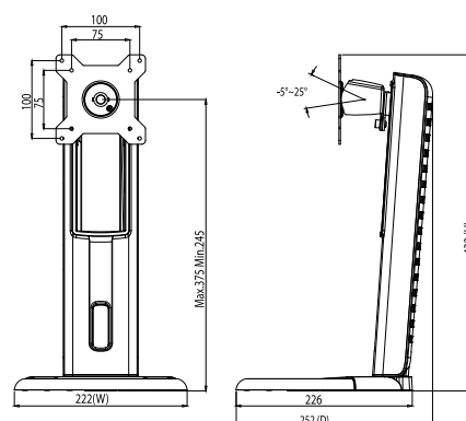
Forward/Backward Tilt (+25°/-5°)
