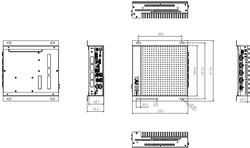
TANK-XM813
