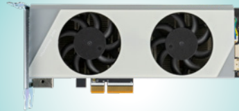
Mustang-V200-KB3 Three Intel® Movidius™ Keem Bay™
